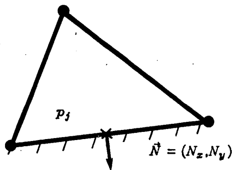
Figure 3 : Boundary Element
