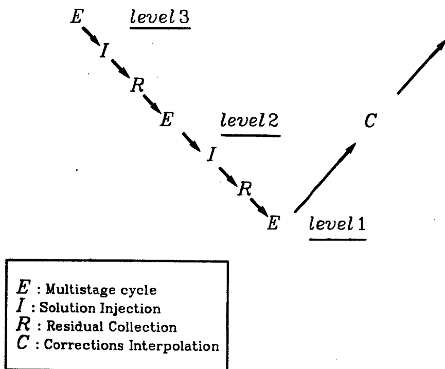
Figure 6 : Multigrid Cycle
