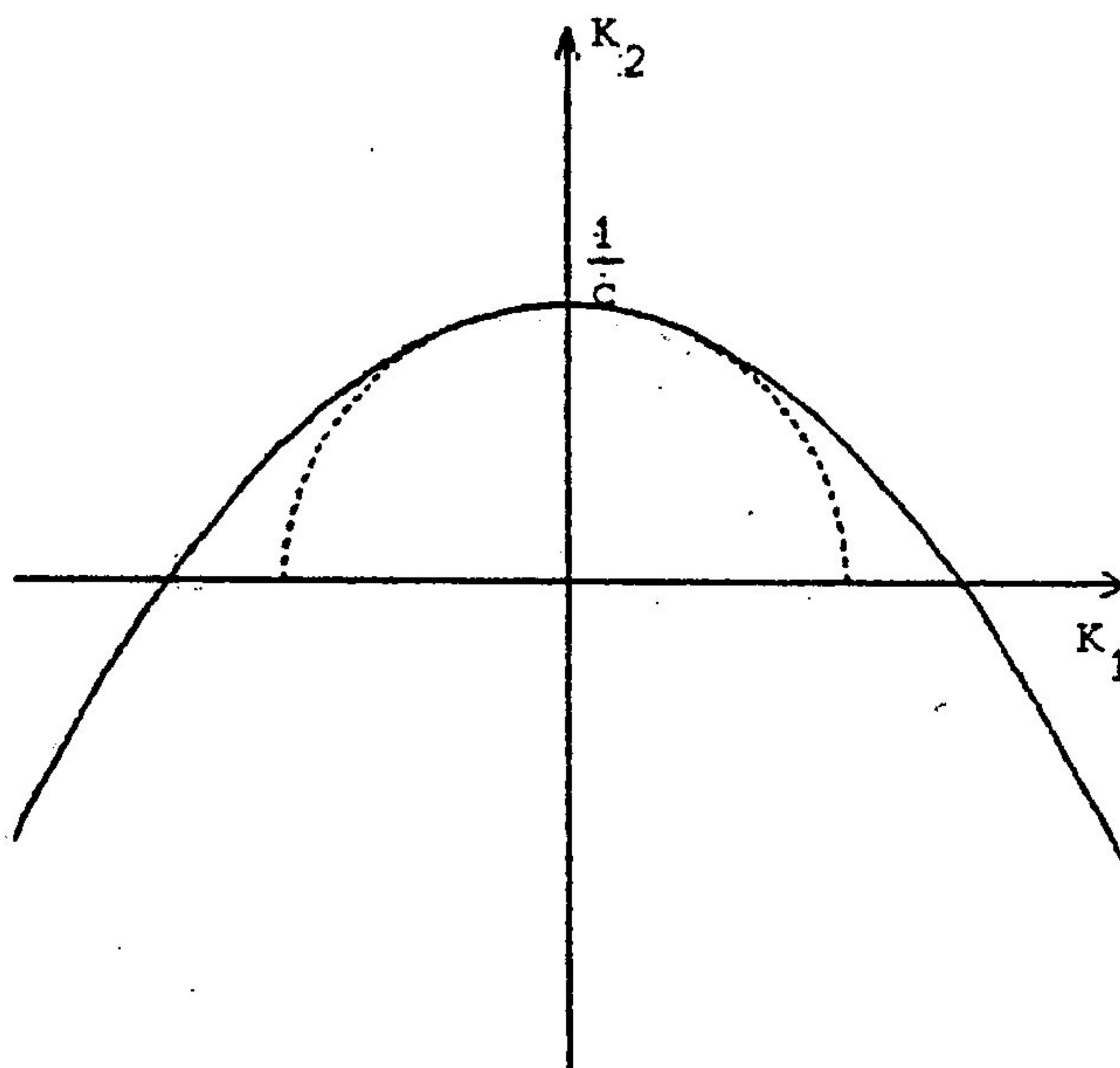
Figure 2.1 : dispersion relations
