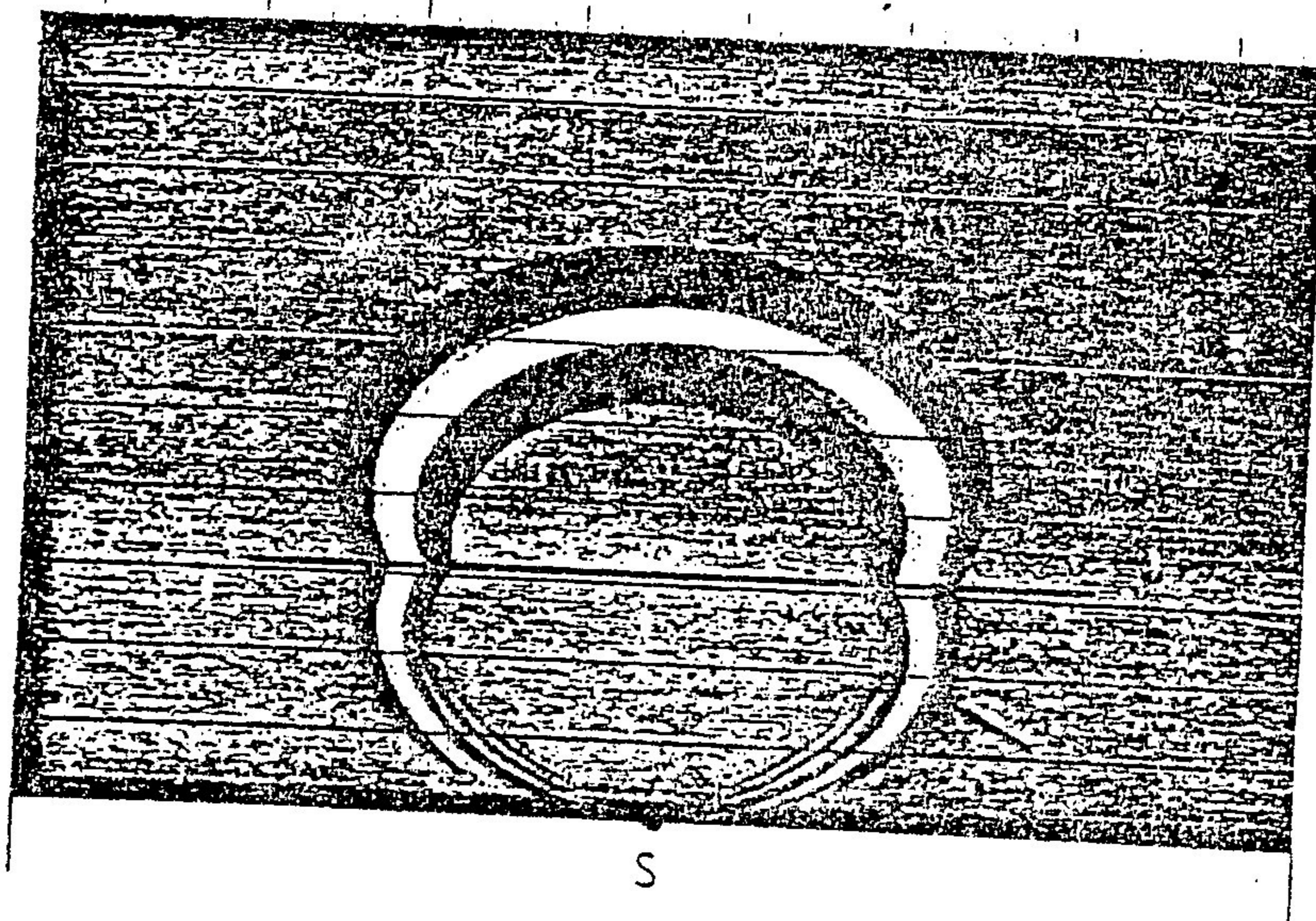
Figure 5.2 : Two-layers medium : horizontal interface
