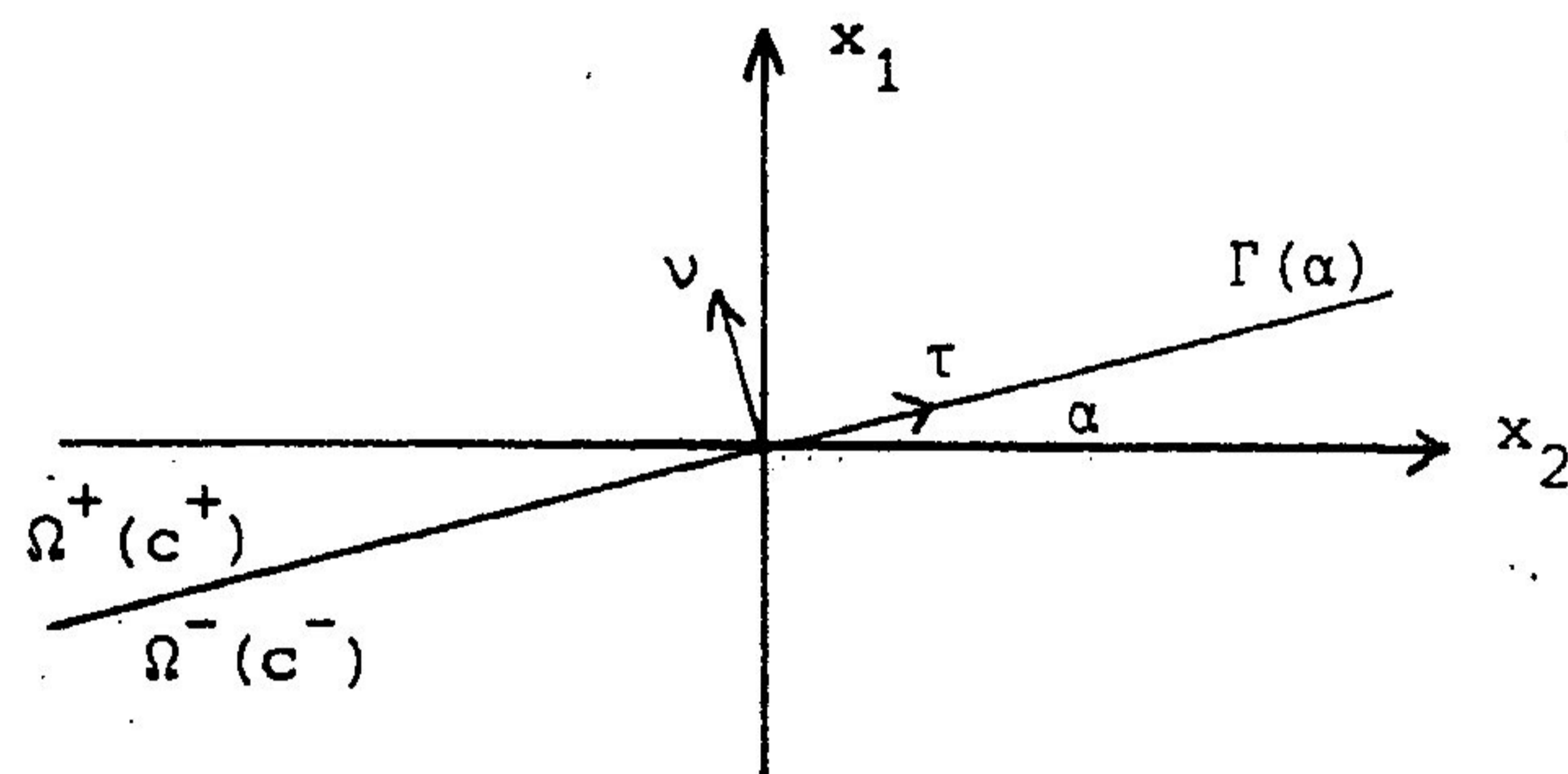
Figure 3.1 : description of the medium
