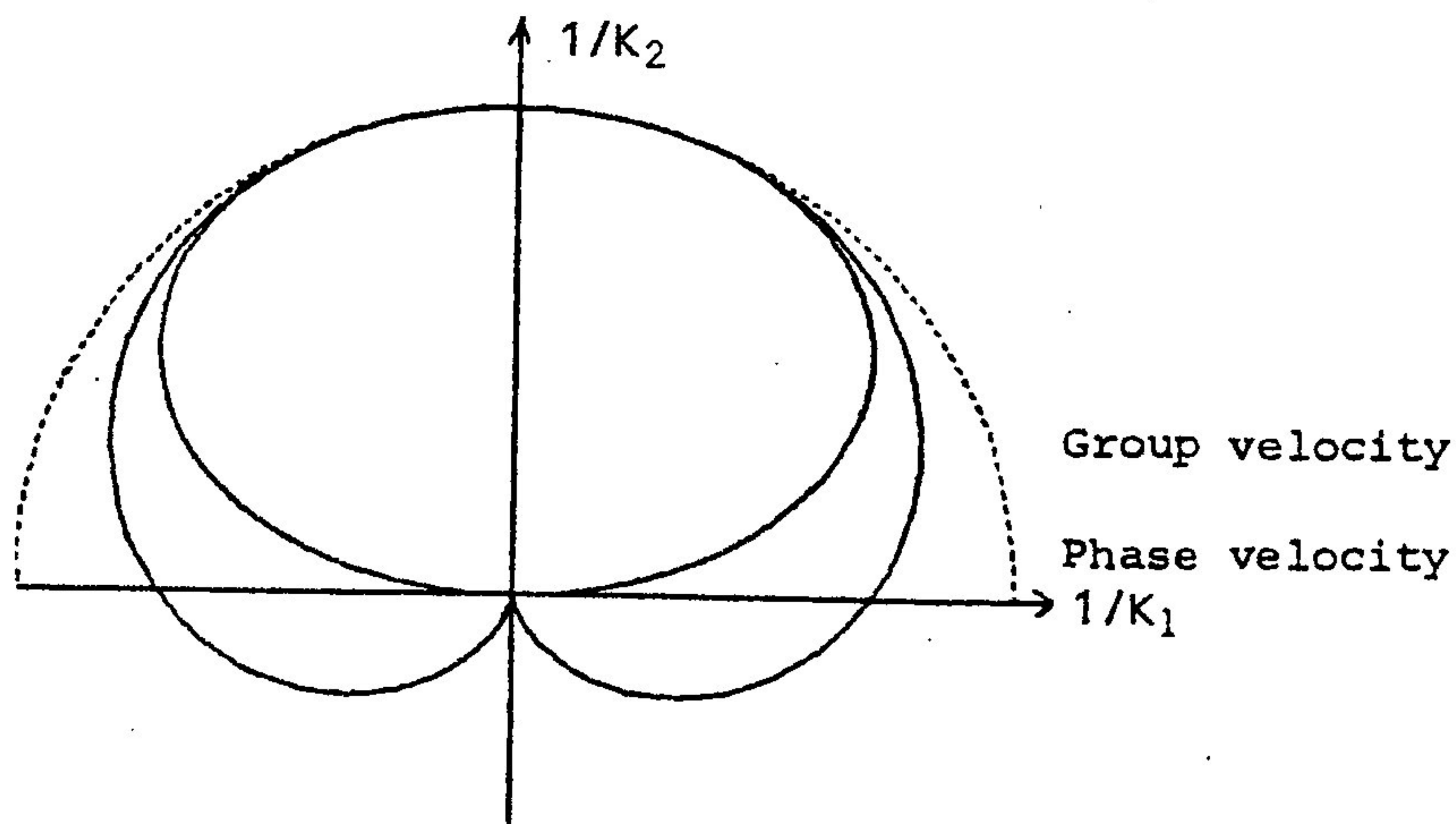
Figure 2.3: phase velocity, group velocity
