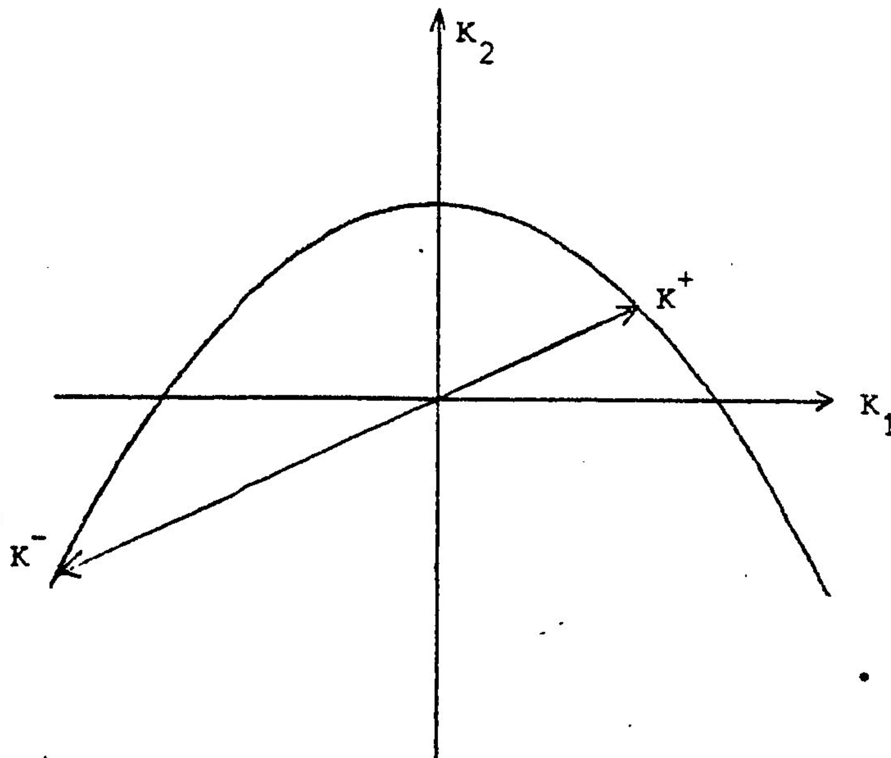
Figure 2.2 : the two propagation modes
