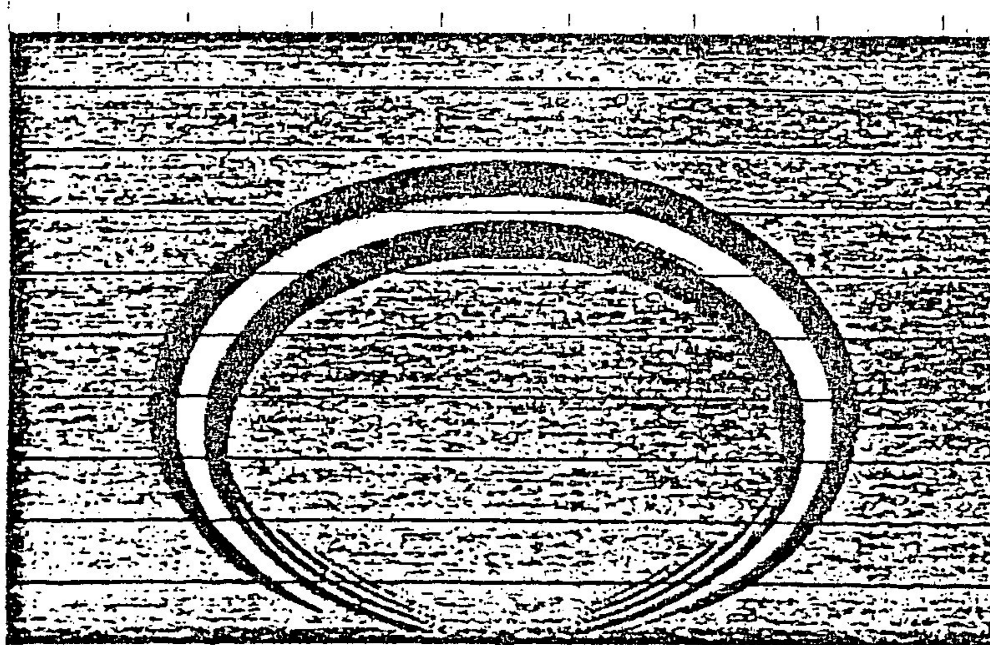
Figure 5.1 : Fundamental solution in homogeneous medium
