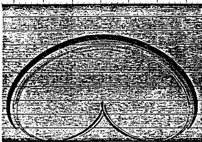
Equation (4.1)
