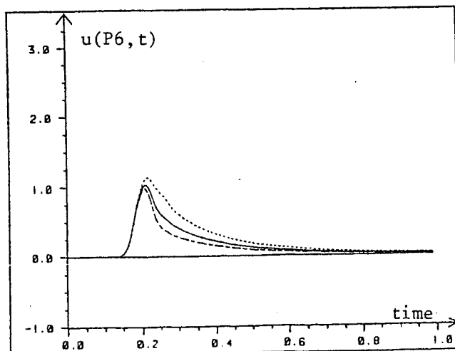
Figure 56: Response at P6=(.99,.99) 2nd order ABC \gamma=1.5 2nd order ABC \gamma=0.1 2nd order ABC \gamma=3.0
