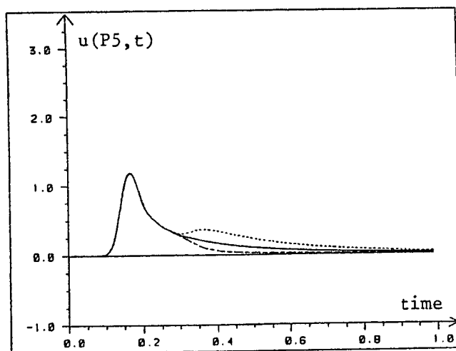
Figure 54: Response at P5=(.99,.89) 2nd order ABC \gamma=1.5 2nd order ABC \gamma=0.1 2nd order ABC \gamma=3.0
