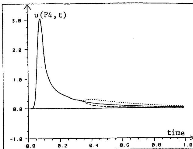
Figure 52: Response at P4=(.89,.89) 2nd order ABC \gamma=1.5 2nd order ABC \gamma=0.1 2nd order ABC \gamma=3.0
