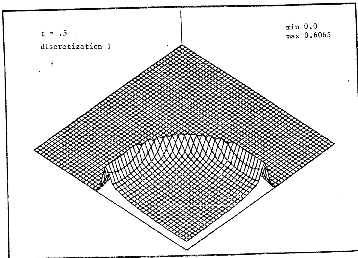
Figure 16: exact solution
