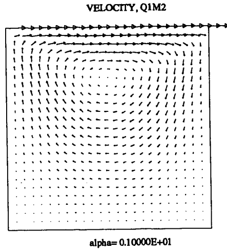
Fig 8: Cavity: "flow through"
