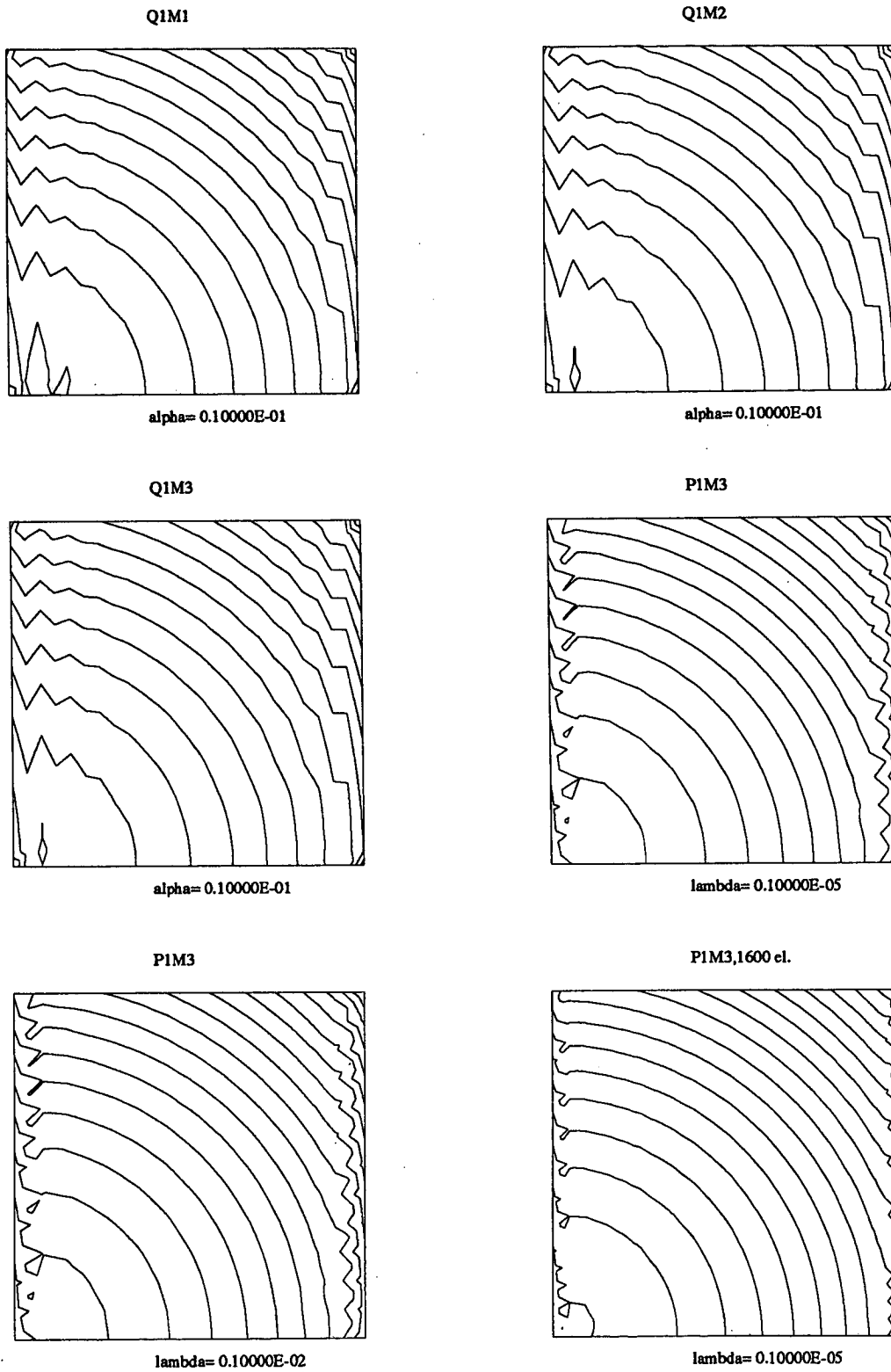
Fig 3: Residual spurious pressures
