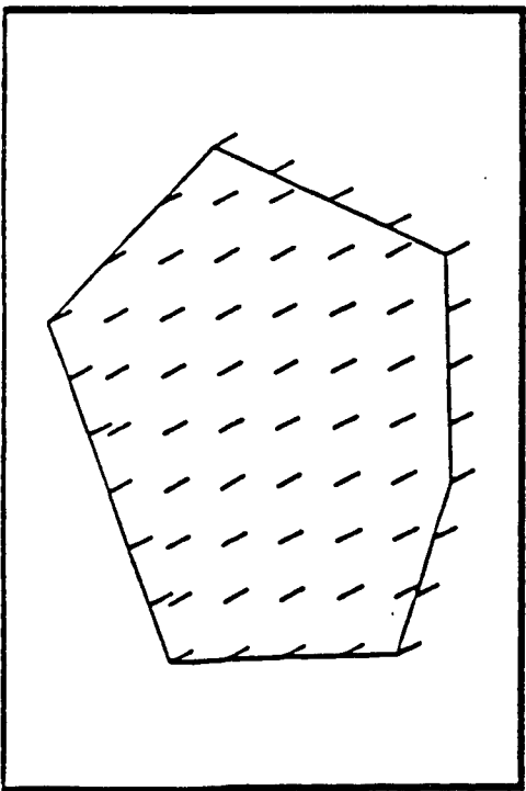
Fig. 8.d: True velocity
