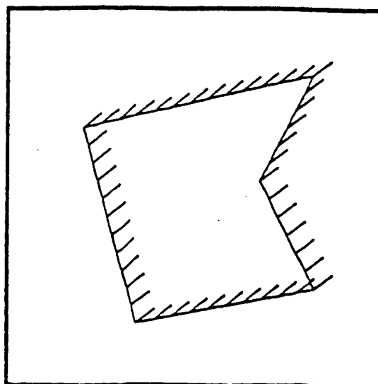
Figure 2.c: Estimated velocity
