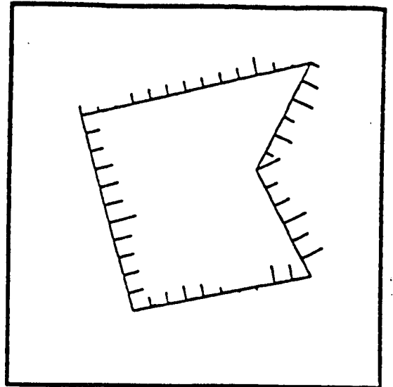
Figure 3.d: Observations, var = 0.1
