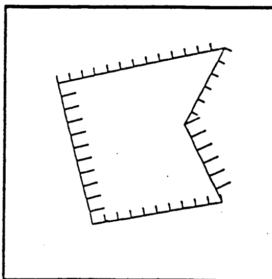
Figure 2.b: Perpendicular component
