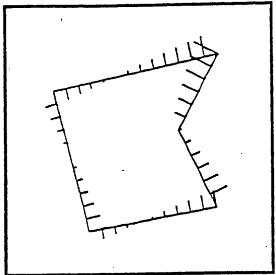
Figure 6.b: Perpendicular component
