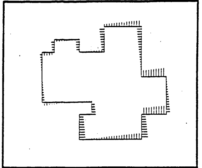
Figure 4.b: Perpendicular component
