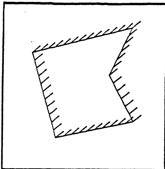
Figure 2.a: True velocity
