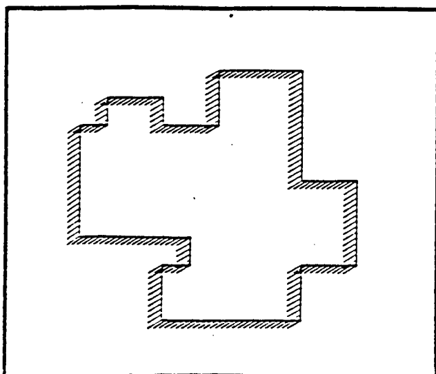
Figure 1.c: Estimated velocity
