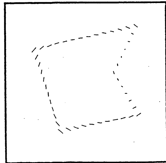
Figure 6.f: Estimation error, a=0.1
