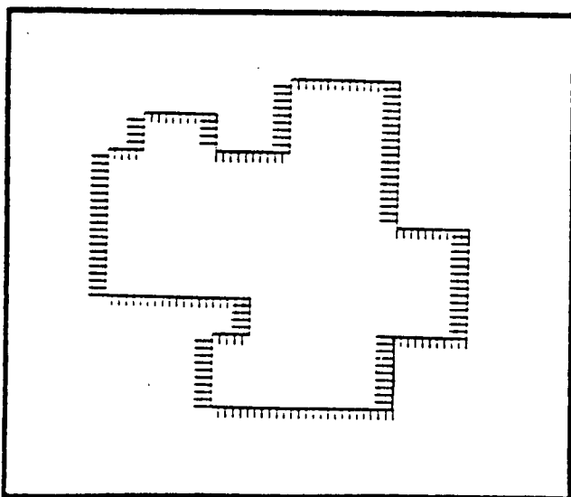
Figure 1.b: Perpendicular component
