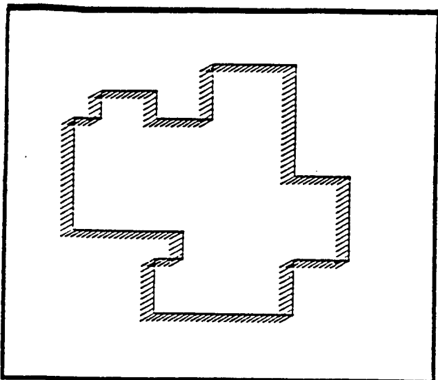
Figure 1.a: True velocity
