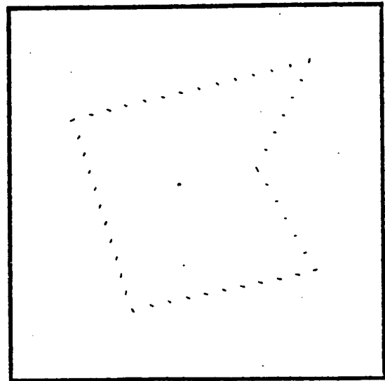
Figure 6.d: Estimation error, a=0.7
