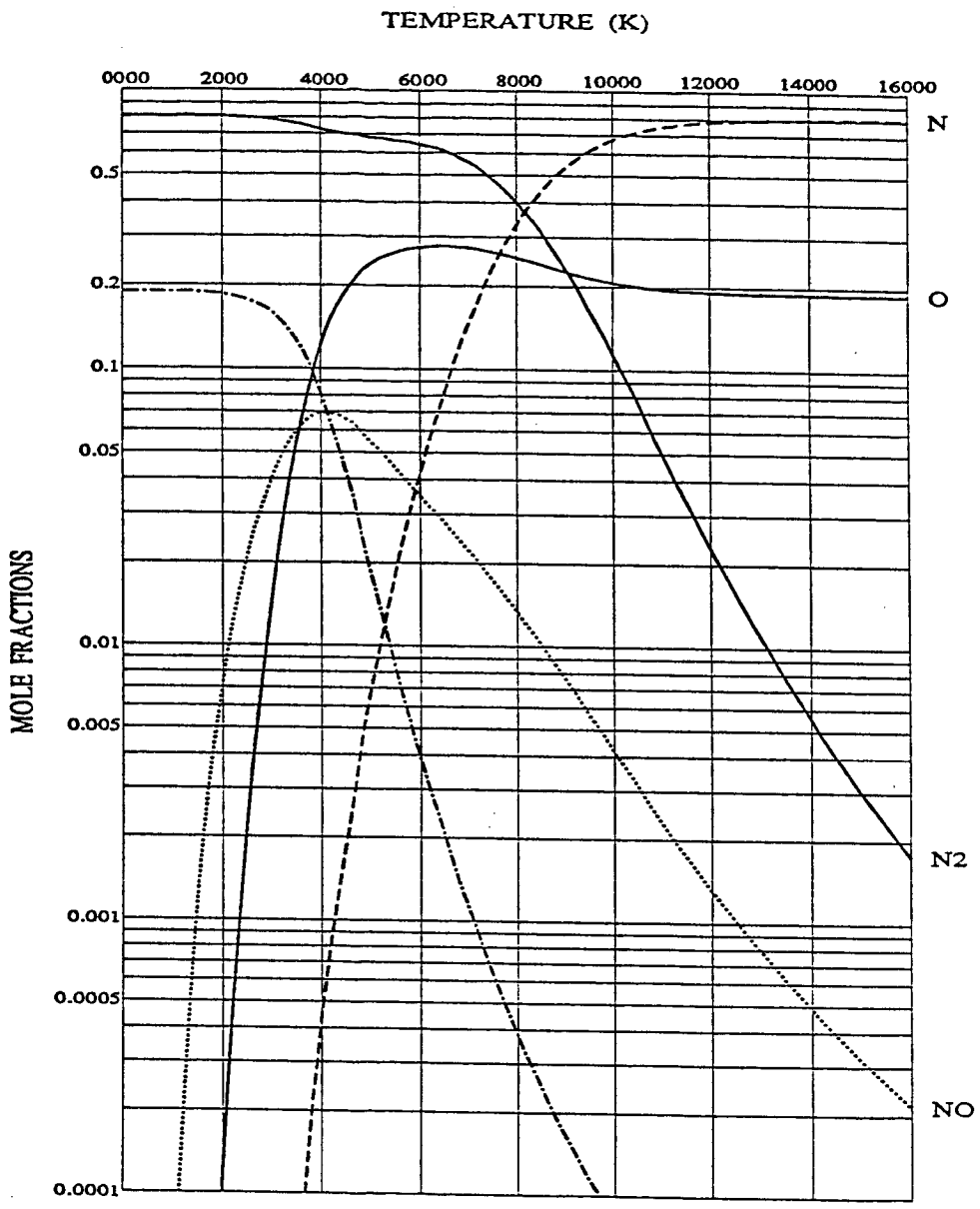
EQUILIBRIUM COMPOSITION OF AIR
