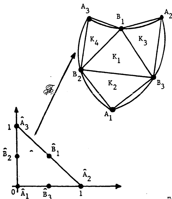
Fig. 4.1. : The reference Lagrange finite element (\hat{\mathcal{K}}, P_2(\hat{\mathcal{K}}), \hat{\mathcal{I}}) and its isoparametrically equivalent finite element (\mathcal{K}, \mathcal{P}, \mathcal{I})
