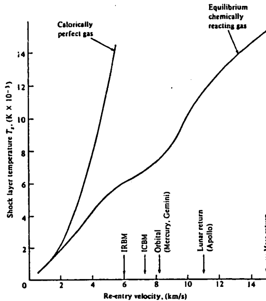
Figure 13.1 Temperature behind a normal shock versus velocity for air at a standard altitude of 52 km. Comparison between calorically perfect and equilibrium gas results.
