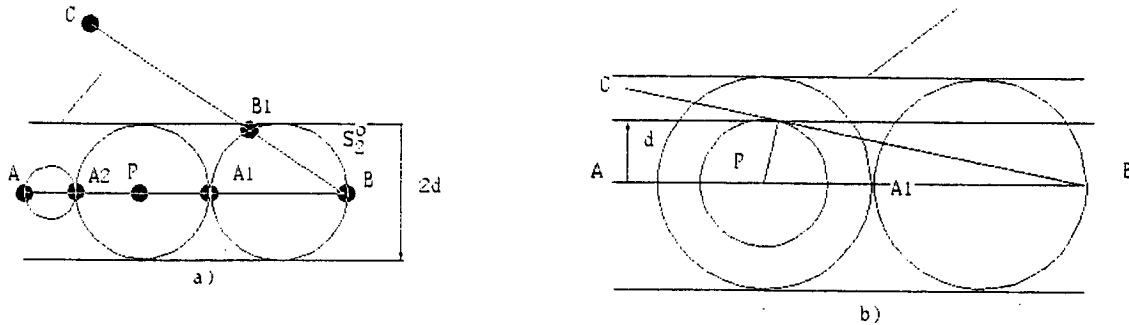
Figure 7: The plane \mathcal{P} perpendicular to AB in B a) separates AB and BC b) does not separates AB from BC
