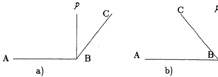
Figure 7: The plane \mathcal{P} perpendicular to AB in B a) separates AB and BC b) does not separates AB from BC
