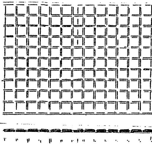
Figure 28: Front and top view of 3D lines when colinearity is discovered and enforced
