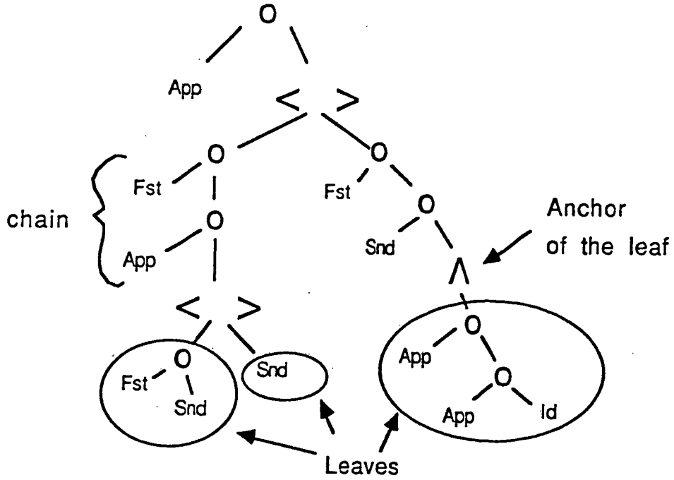
Figure 7: A term in \mathcal{E} -normal form
