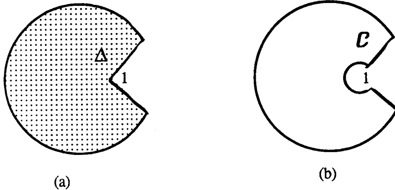
Figure 1. (a) The domain \Delta(\phi, \eta) . (b) The contour \mathcal{C} used in the proof of Theorem 1.
