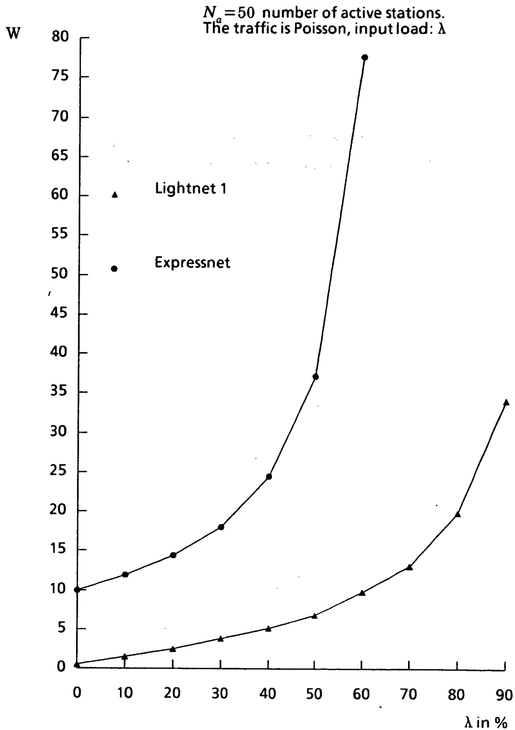
Figure 7: Comparison between Expressnet and Lightnet 1. Average delay versus input load \lambda .
