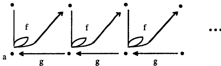
Fig 2.1. Hypergraphe.
