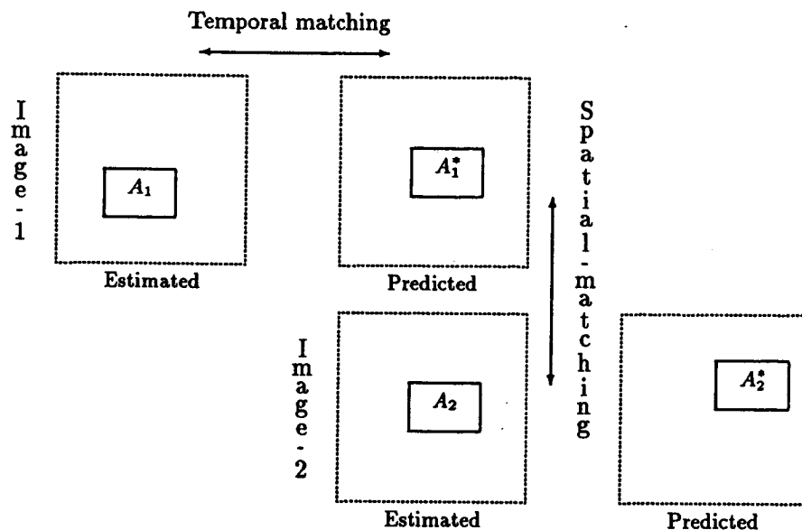
Figure 8 : Temporal and Spatial Matching of 2D line Segments
