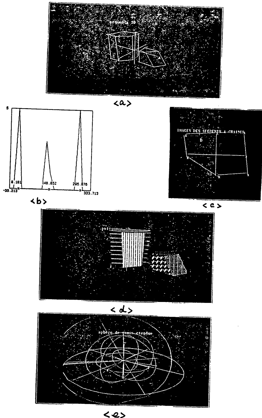
Figure 20 : The identification of 3D polygons. It is shown : (a) the set of 3D line segments with about 5% errors; (b) an exemple of the estimation of the parameters \rho ; (c) an exemple of the linking of 3D line segments; (d) the estimated 3D polygons; (e) the representation of the estimated 3D polygons in the Extended GAUSS Sphere.
