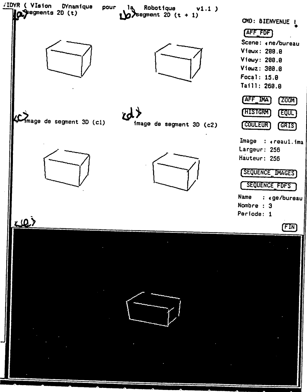
Figure 19 : The triangulation of 3D line segments: (a) and (b) the matched 2D line segments in two images; (c) and (d) the projection of the estimated 3D line segments to the camera at two different positions; The figure below is the 3D visualization of the 3D line segments.
