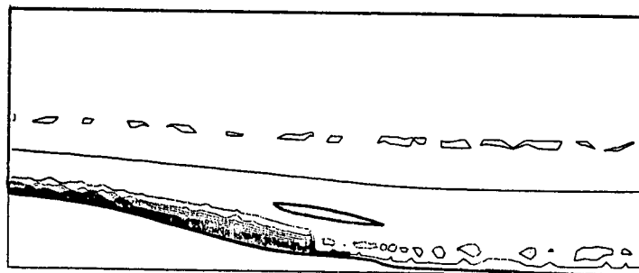
Figure 12. The vorticity \left(\frac{\omega_\theta}{r}\right) field of the stationary solution computed by our iterative method in the case of a duct propeller.
