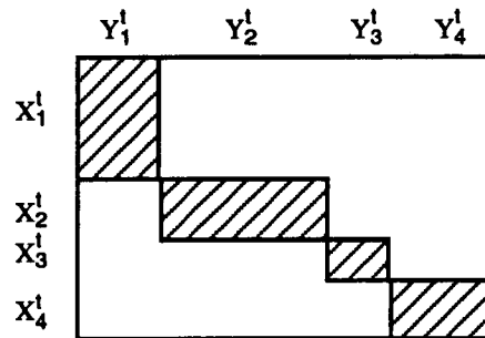
Figure 1. The diagonal blocks formed by one-to-one related subsets of product and machine types maximize the criterion \Delta .
