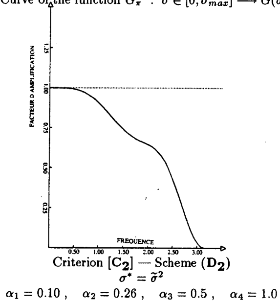
Figure 15: Curve of the amplification factor \theta \in [0, \pi] \rightarrow G(\sigma^*, \theta, \alpha_1, \alpha_2)
