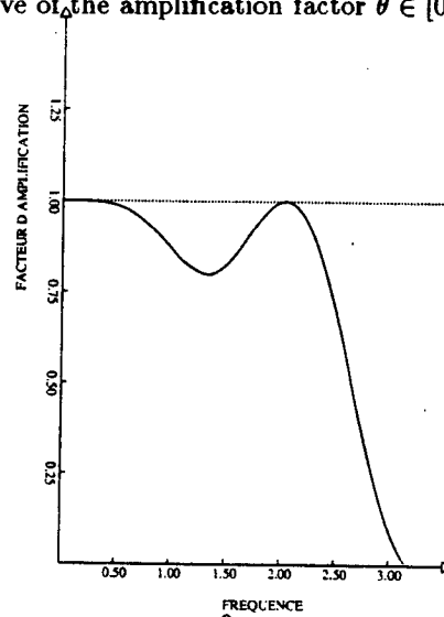
Figure 27: Curve of the amplification factor \theta \in [0, \pi] \rightarrow G(\sigma, \theta, \alpha_1, \alpha_2)
