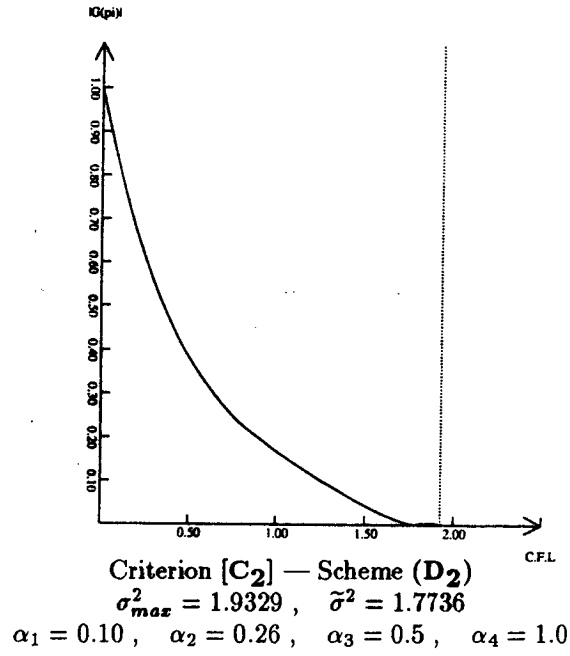
Figure 14: Curve of the function G_\pi : \sigma \in [0, \sigma_{max}] \rightarrow G(\sigma, \pi, \alpha_1, \alpha_2) .
