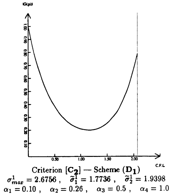
Figure 12: Curve of the function G_\pi : \sigma \in [0, \sigma_{max}] \rightarrow G(\sigma, \pi, \alpha_1, \alpha_2) .
