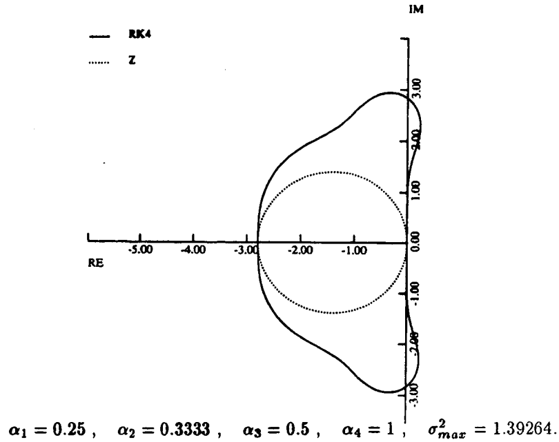
Figure 6: RK4 stability domain with (D_1) as spatial approximation.
