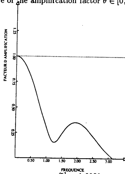
Figure 23: Curve of the amplification factor \theta \in [0, \pi] \rightarrow G(\sigma, \theta, \alpha_1, \alpha_2)
