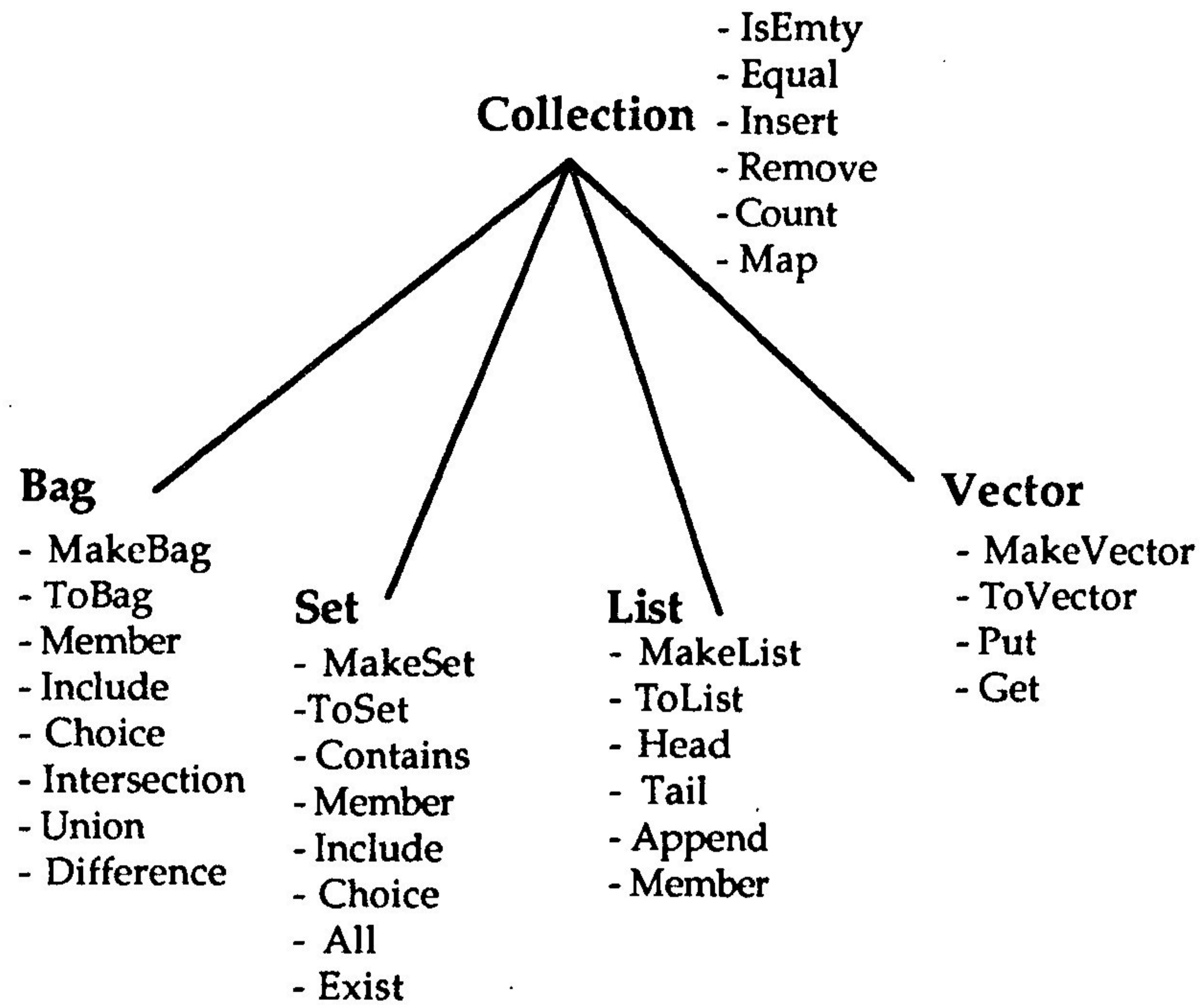
Figure 1 : The Collection generic ADT hierarchy.
