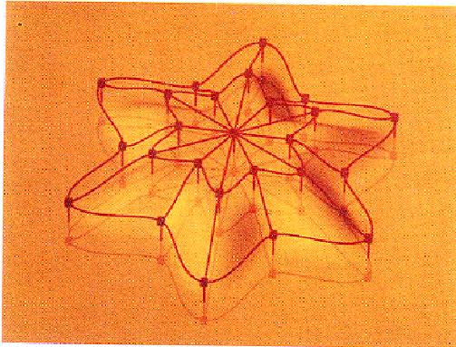
Figure 6b: The deformed lattice and the deformed surface
