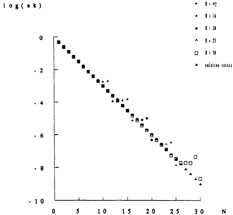
Fig. 4.1 b. Spectral coefficients of the solution, with \tilde{\lambda}
