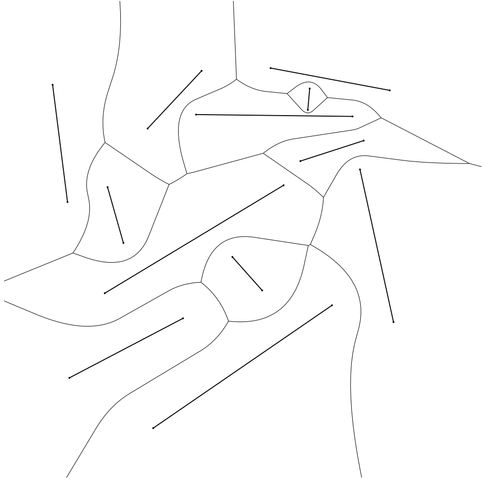
Figure 3: Example of Voronoi diagram of line segments
