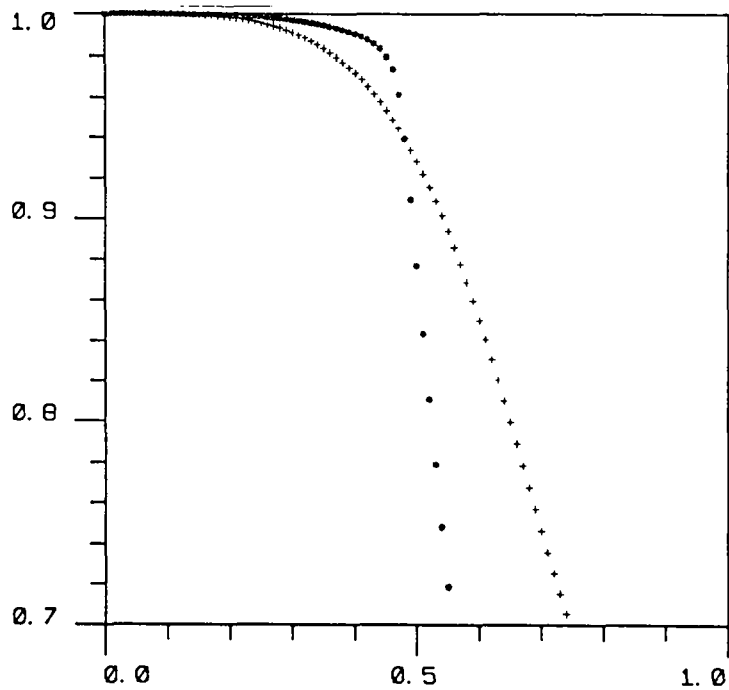
Figure 6.7: Phase speed: + ↔ c = 0 and \alpha = 1.5 ; * ↔ c = 0.207 and \alpha = 2.13 .
