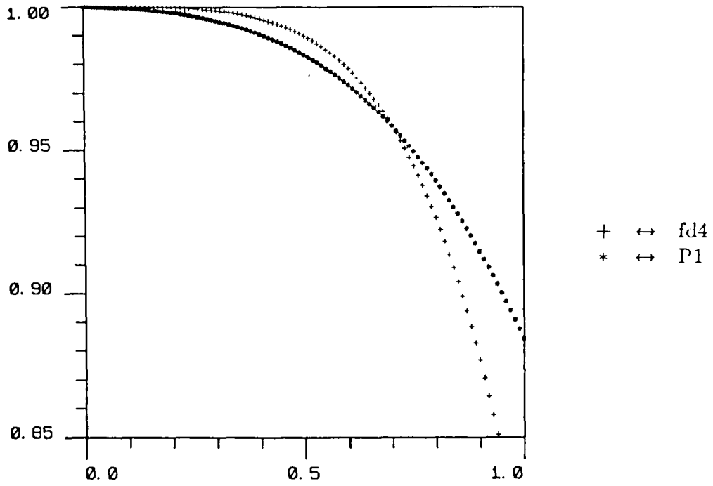
Figure 5.4: Phase speed; \varphi = \theta = 0
