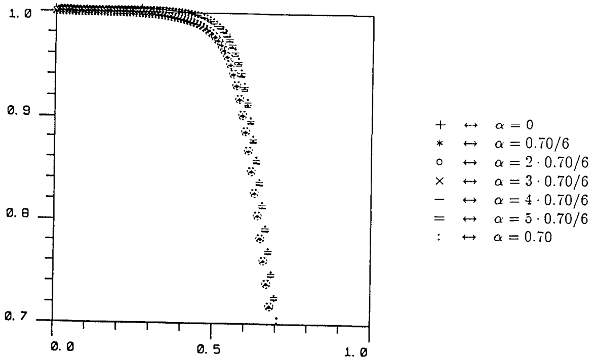
Figure 4.2: The phase speed for P2 elements
