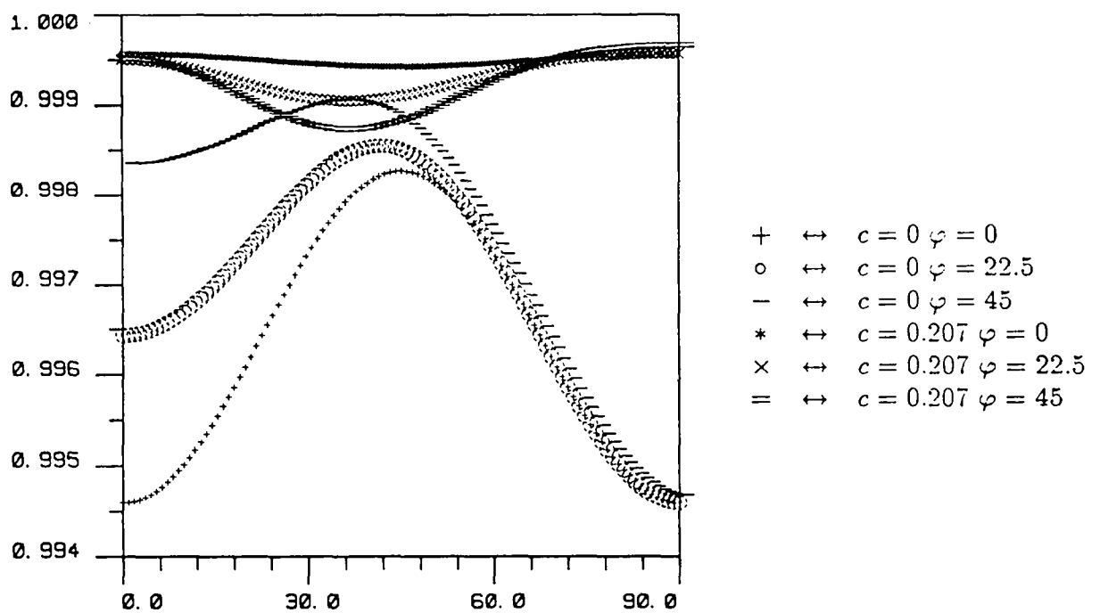
Figure 6.9: Phase speed without scaling, N = 10 .
