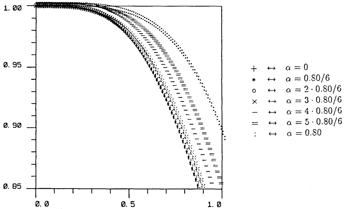
Figure 5.2: Phase speed; \varphi = \theta = 45
