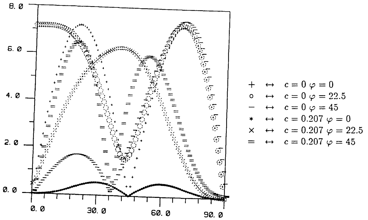
Figure 6.12: Error in the direction of propagation, N = 5
