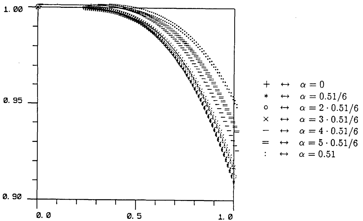
Figure 5.3: Phase speed; \varphi = \theta = 45
