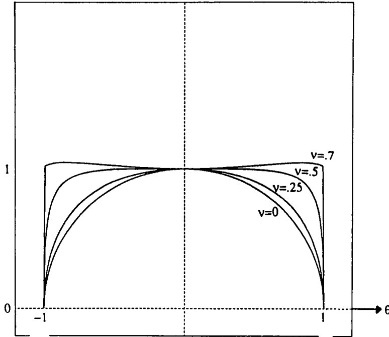
Figure 3. The functions r(\theta) for \nu_p=1 and \nu=0, 1/4, 1/2 , and \sqrt{2}/2 .
