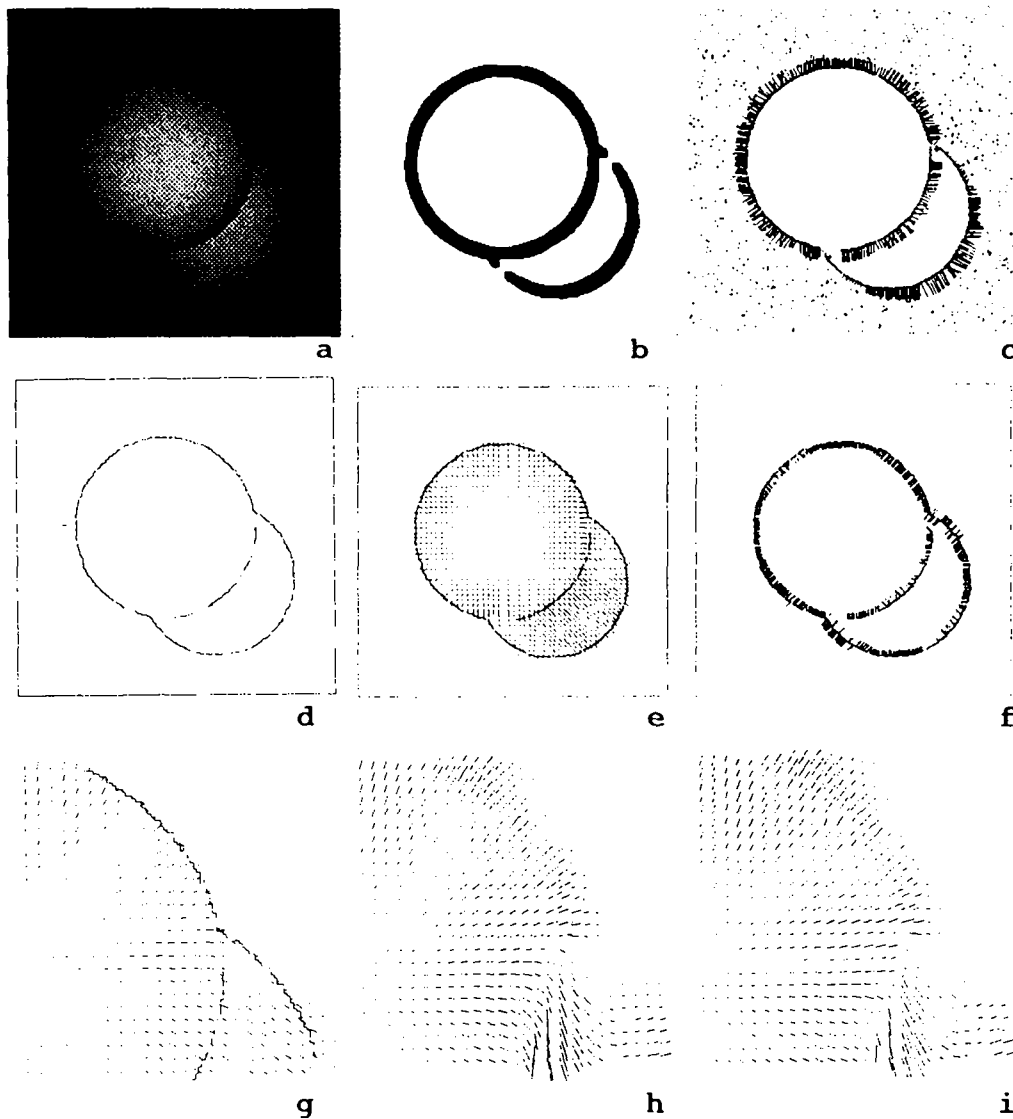
Figure 10 : motion estimation on the moving disks sequence.
