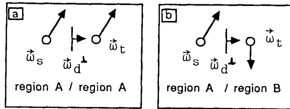
a) moving edge within a region b) occluding edge between two regions | : moving edge site O : pixel site
