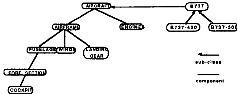
Figure 1. Composite objects.
