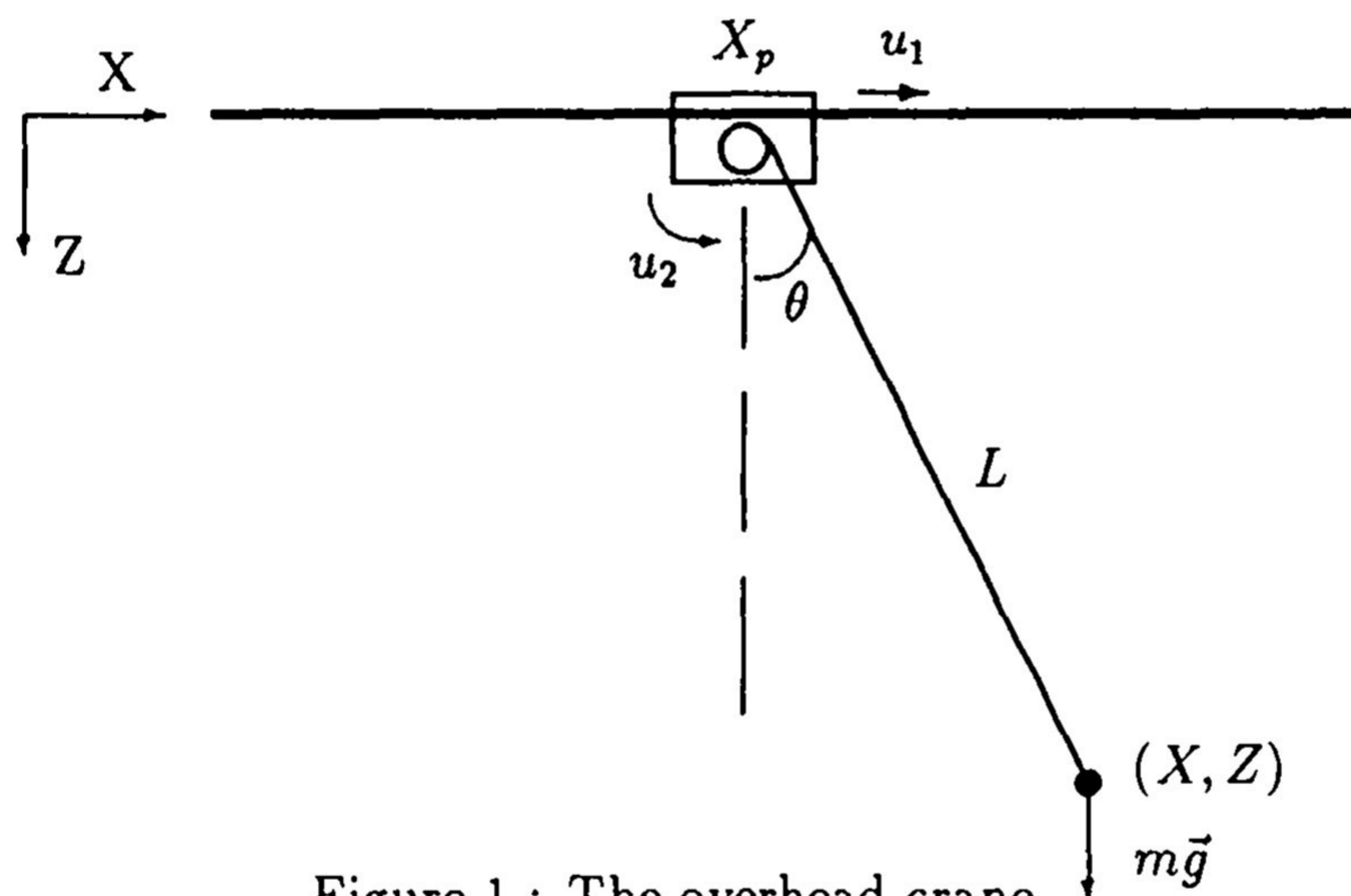
Figure 1 : The overhead crane
