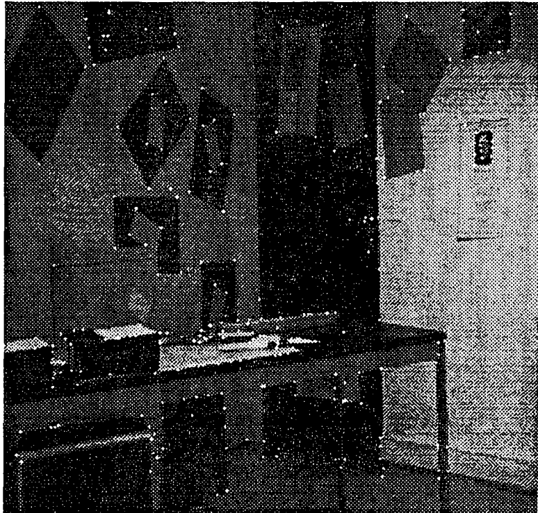
Figure 21: Corners points detected on an indoor scene
