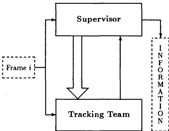
Fig. 2: An Architecture for Motion Tracking
