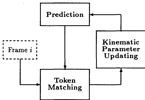
Fig. 3: Block Diagram of the Token Tracking Algorithm
