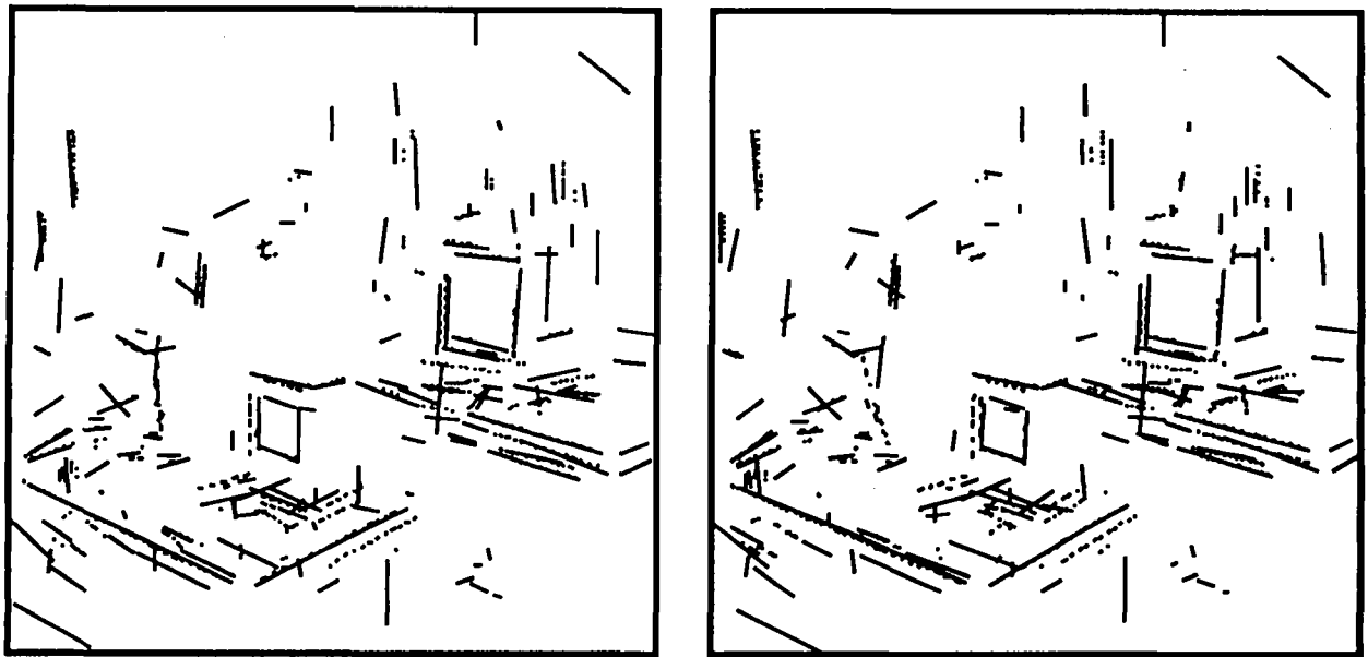
Fig. 19: A stereogram showing the superposition of the predicted (in solid lines) and observed (in dashed lines) segments at t_{15}
