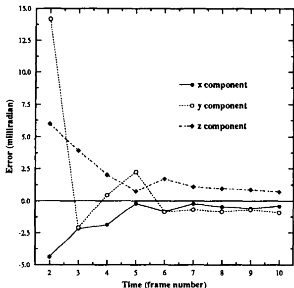
Fig. 13: Error evolution in the angular velocity of the rotating table undergoing general motion
