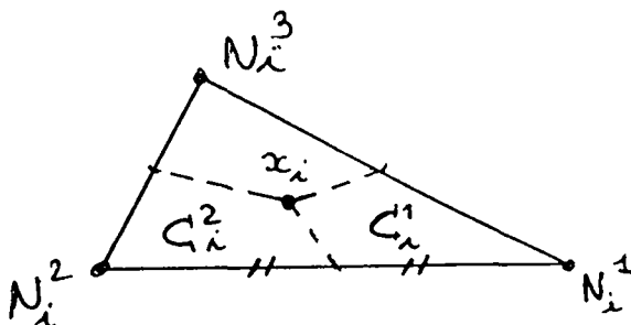
Figure 2. Subcell decomposition for a triangular mesh.
