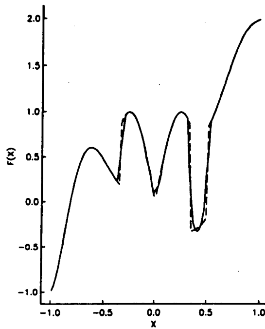
Figure 3.12: Cross-section at Y = 0 of the E.N.O interpolation (a) and the E.N.O. reconstruction (b) for 1600 nodes the mesh. 46
