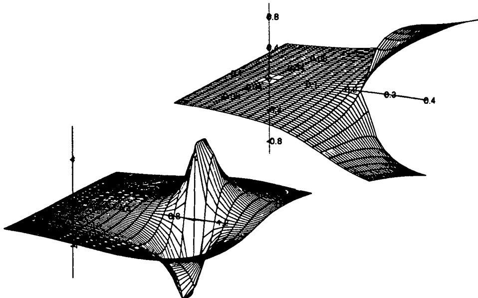
Figure 2. A display of the imaginary parts of two generating functions,
