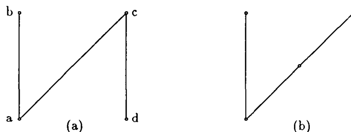
Figure 4: (a) The HASSE-diagram of the poset "N" ; (b) an N-free poset
