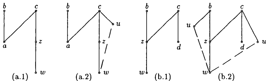
Figure 7: Case 1: z = d ; Case 2: z = a
