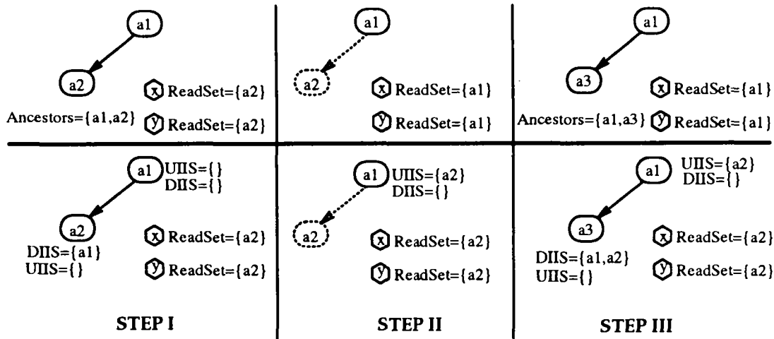
Figure 2: Upward and Downward Inheritance Example
