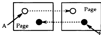
Figure 1: False Deadlock
