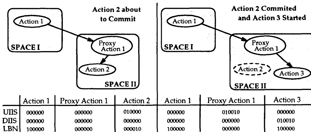
Figure 3: Upward Inheritance of Locks
