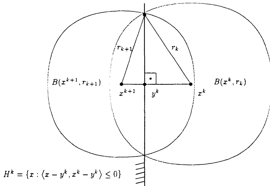
Figure 2.1: Illustration of the Fejér property of x^{k+1} = x^k + t_k(y^k - x^k) with y^k = P_{H^k}(x^k) when x^{k+1} \in S . By Pythagoras' theorem, r_{k+1}^2 - |x^{k+1} - y^k|^2 = r_k^2 - |y^k - x^k|^2 , where x^{k+1} - y^k = (t_k - 1)(y^k - x^k) , so r_{k+1}^2 = r_k^2 - t_k(2 - t_k)|y^k - x^k|^2 . Clearly, B(x^k, r_k) \cap H^k \subset B(x^{k+1}, r_{k+1}) \cap H^k .
