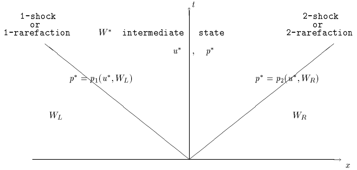
Figure 34 : The solution of Riemann problem
