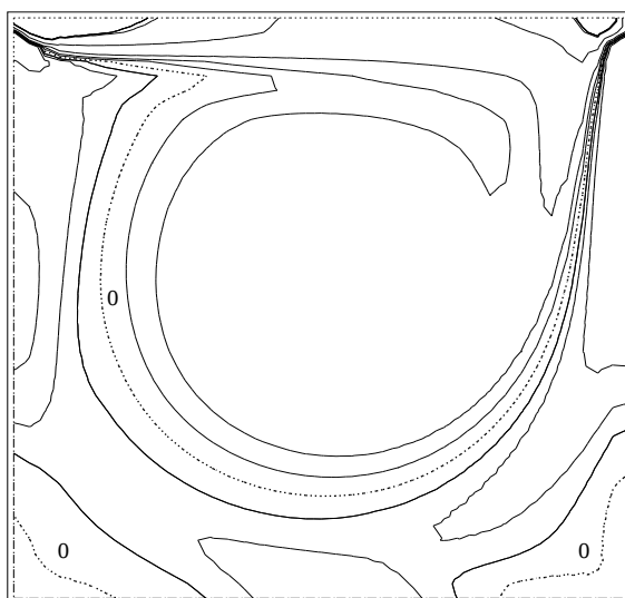
Figure 26 : Lines of equivorticity for Re = 1000 (41 x 41 nodes mesh)
