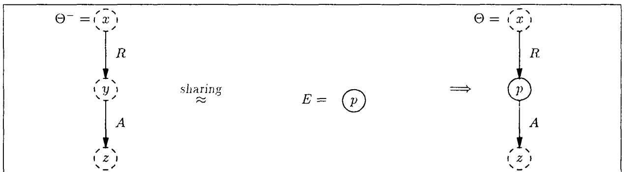
Figure 6: An ill-formed signature
