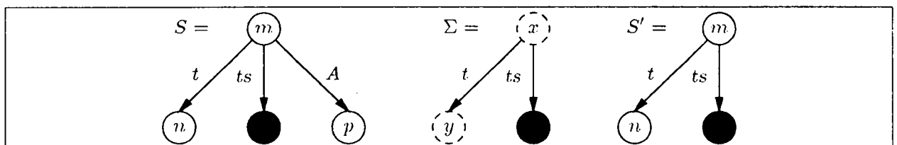
Figure 2: Representation of S , S' and \Sigma
