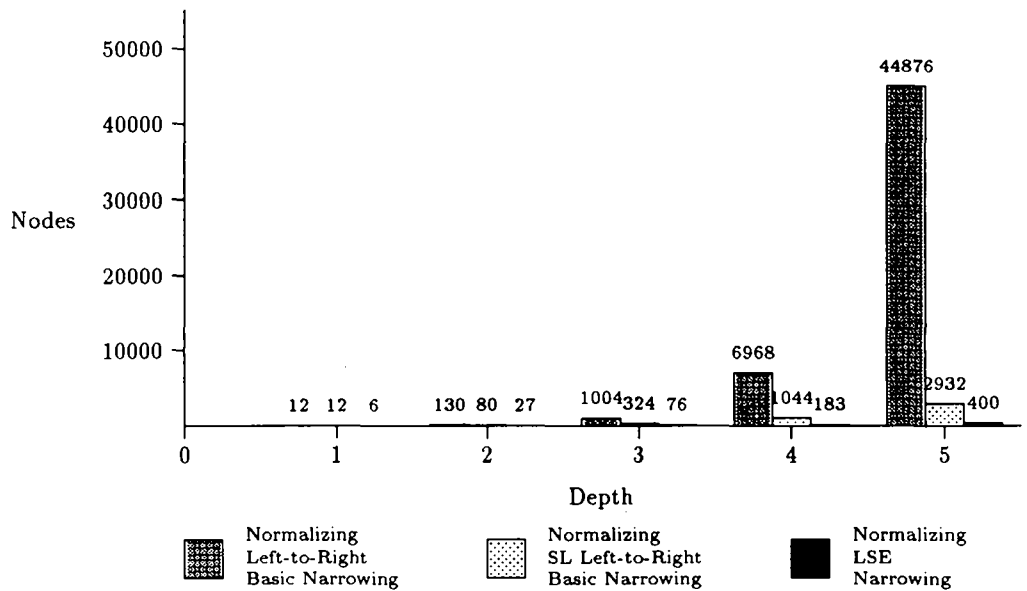
Fig. 5. Best narrowing strategies for arbitrary systems (only normalized substitutions)
