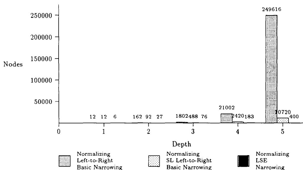
Fig. 6. Best narrowing strategies for arbitrary systems (all substitutions)
