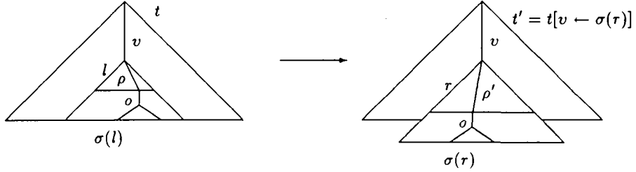
Fig. 2. Illustration of antecedents: the occurrence v.\rho.o is an antecedent of v.\rho'.o .
