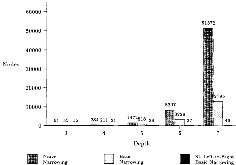
Fig. 3. Non-normalizing strategies
