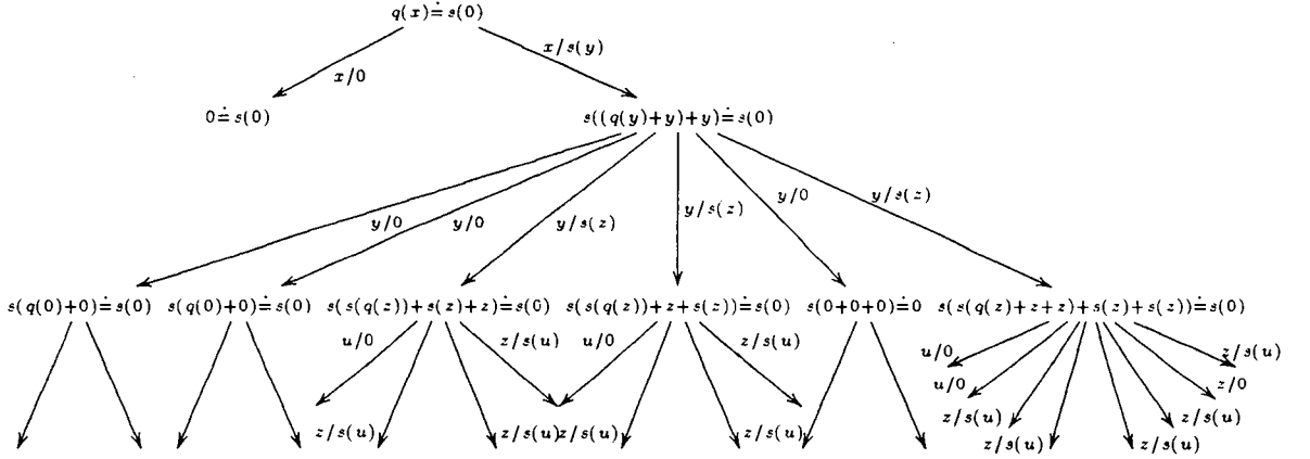
Fig. 1. Narrowing tree for q(x) \doteq s(0)
