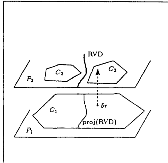
Figure 1.8: Connecting contours between adjacent cross-sections by calculating the region Voronoi diagram (RVD) and linking infinitesimal surfaces to the closest point.
