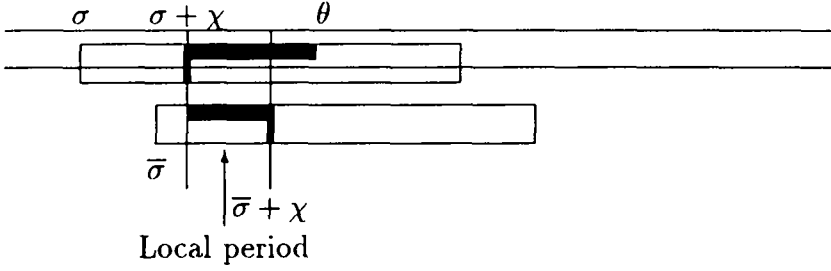
Figure 3: Applying critical factorizations. If T[\sigma + \chi.. \theta - 1] = \mathcal{P}[\chi + 1.. \theta - \sigma] and there is an occurrence of the pattern at text position \bar{\sigma} , \sigma < \bar{\sigma} \leq \theta - \chi , then the factorization (\mathcal{P}[1.. \chi], \mathcal{P}[\chi + 1.. m]) has a local period of length \bar{\sigma} - \sigma .
