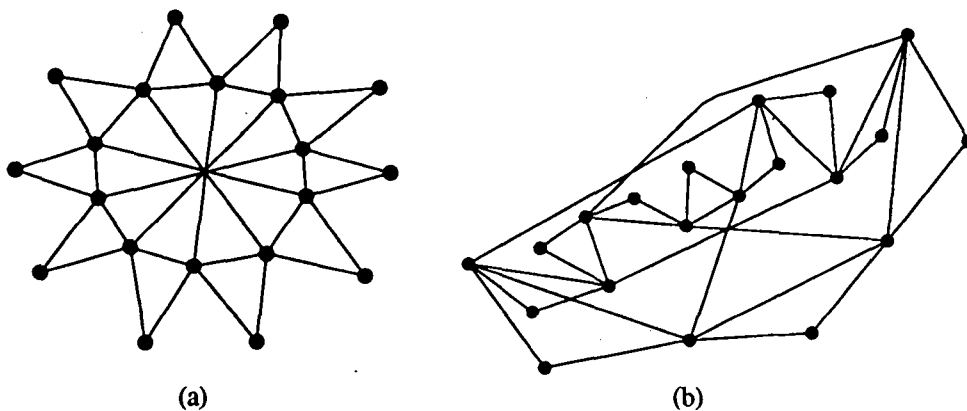
Figure 14: Symmetry vs. planarity.
