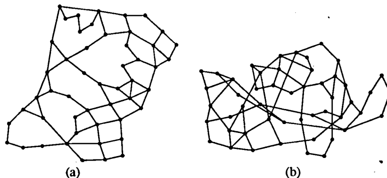
Figure 10: A sparse planar graph: (a) our system's output, and (b) that of the annealing system of [DH89].
