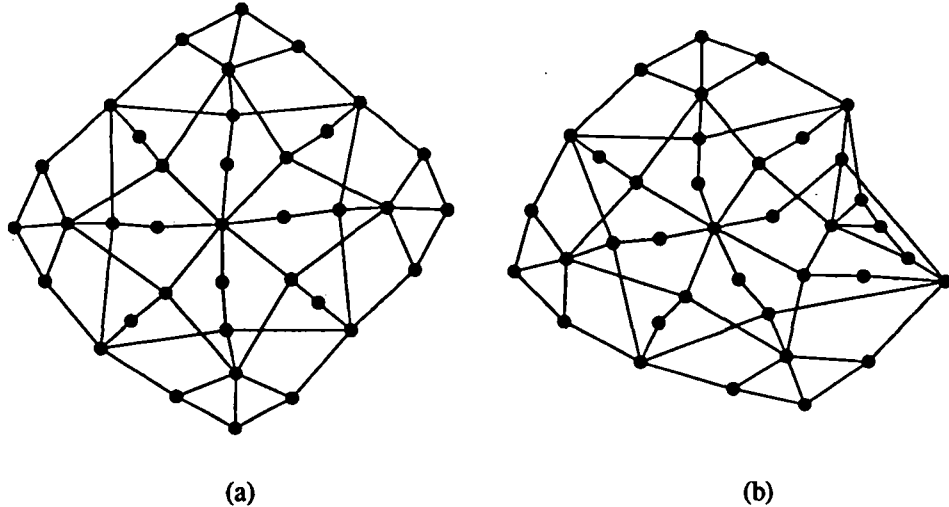
Figure 13: A less lucky example of a nonplanar graph: (a) a hand-drawn version, and (b) our system's output.
