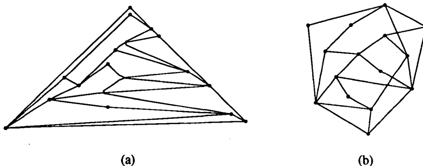
Figure 6: A graph drawn using the shortest face-path heuristic.
