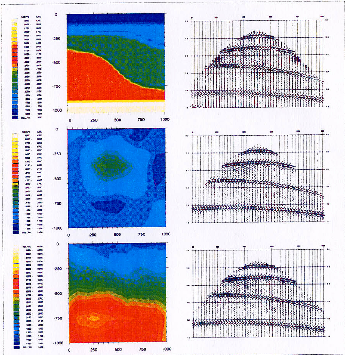
Fig. 4.5 No unique global minimum with respect to the propagator \alpha . Left: velocities, right: corresponding resimulations with the true time reflectivity \mathcal{R} . Top: true velocity. Middle: after 15 hours of multiscale optimization on a Cray-2 from initial guess 1800 m/s. Bottom: after 15 hours of multiscale optimization on a Cray-2 from initial guess 2500 m/s.
