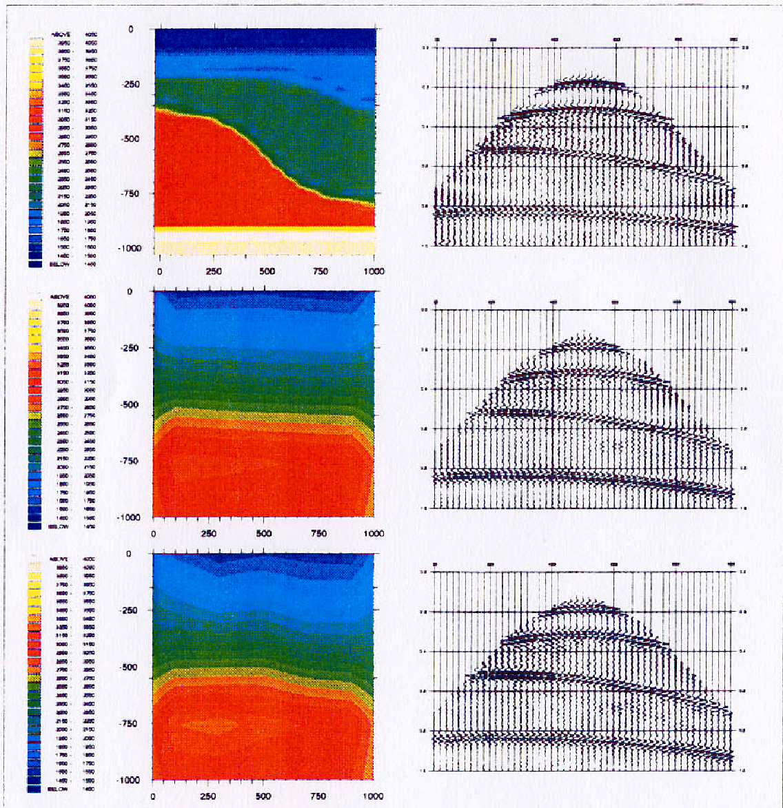
Fig. 4.2 Multiscale minimization with respect to v , with the true time reflectivity s(t) . Top: true velocity v , and data d = \varphi(v, \sigma) = \mathcal{M}\varphi(v, \bar{s}) . Then, left: velocities, and right: corresponding resimulations. Middle: after 3 hours of minimization on a Cray-2 on the 1st scale from the minimum on the 0th scale. Bottom: after 3 hours of minimization on a Cray-2 on the 2nd scale from the minimum on the 1st scale.
