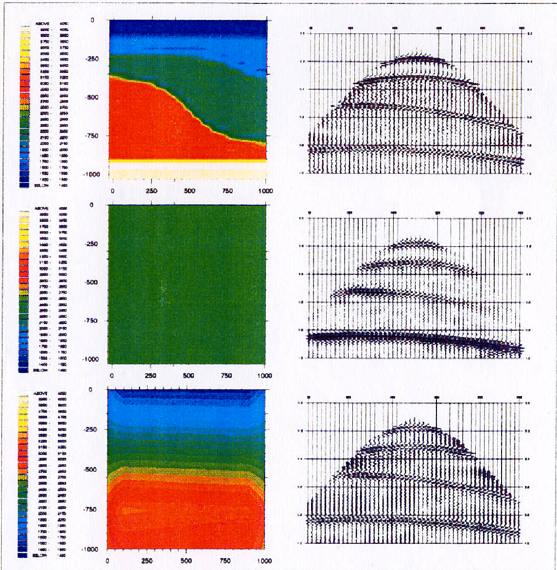
Fig. 4.1 Multiscale minimization with respect to \rho , with the true time reflectivity s(t) . Top: true velocity \bar{\rho}_t , and data d = \varphi(\rho, \sigma) = \mathcal{M}\varphi(\bar{\rho}, s) . Then, left: velocities, and right: corresponding resimulations. Middle: uniform initial guess 2500 m/s. Bottom: after 3 hours of minimization on a Cray-2 on the 0th scale from the initial guess.
