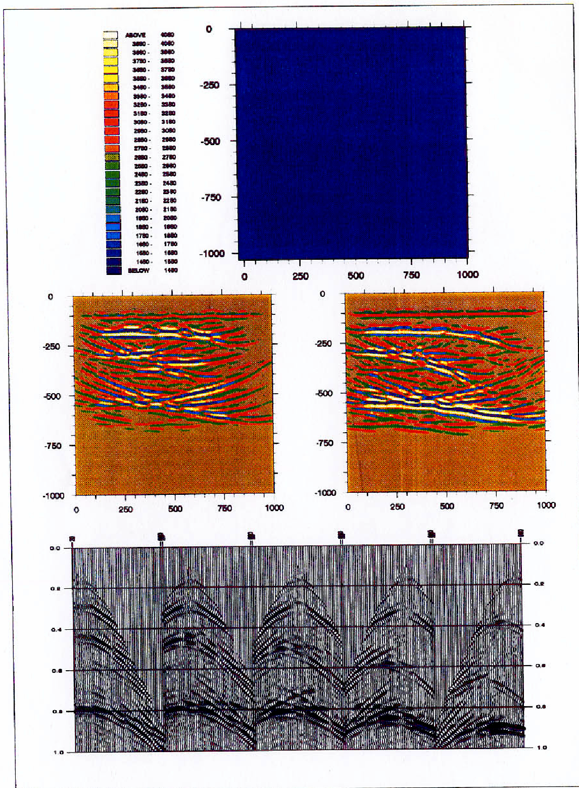
Fig. 5.3 Multishot resimulation with a uniform propagator of 1500 m/s. Top: uniform propagator 1500 m/s. Middle: intermediate stacked depth reflectivity with respect to v (left) and \sigma (right). Bottom: corresponding resimulation.
