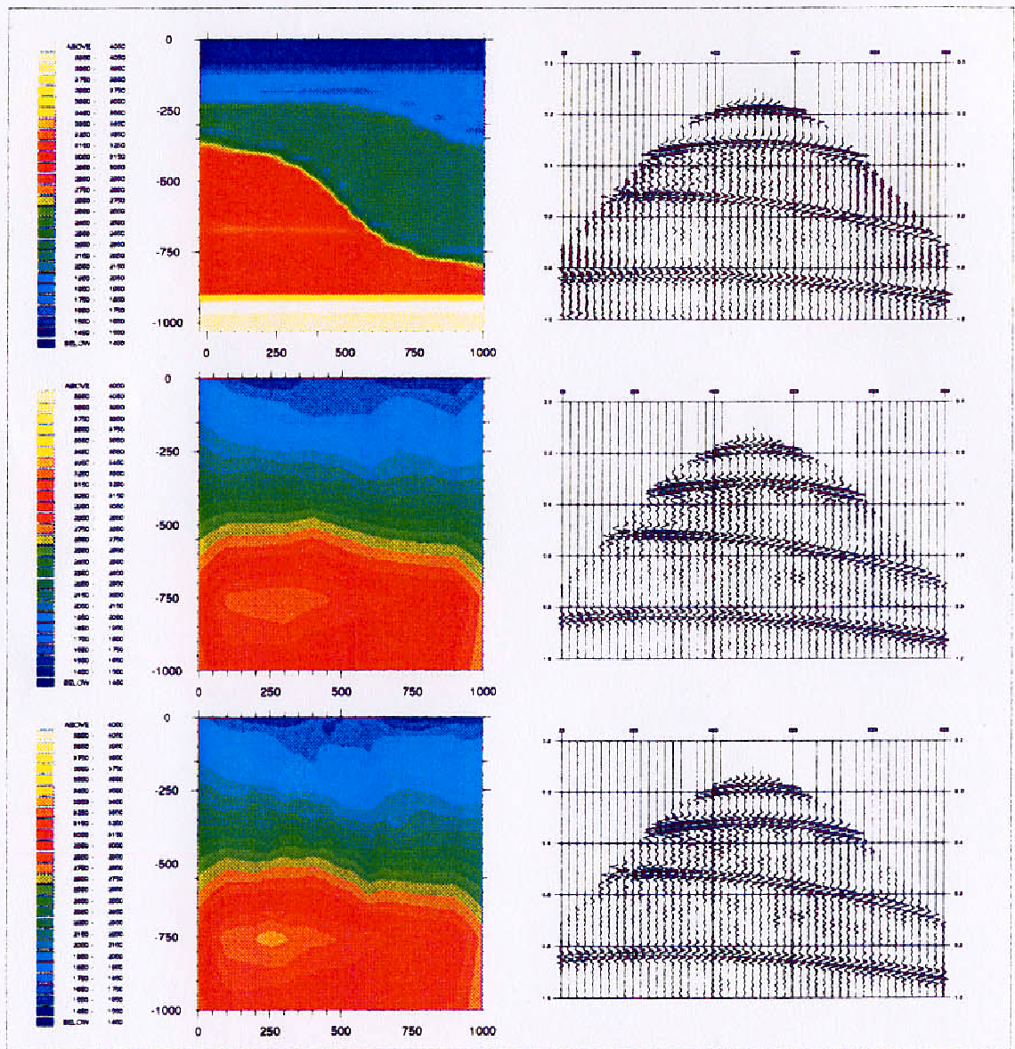
Fig. 4.3 Multiscale minimization with respect to c , with the true time reflectivity s(\delta) . Top: true velocity c , and data d = \varphi(\rho, \sigma) = \mathcal{M}\varphi(\rho, s) . Then, left : velocities, and right: corresponding resimulations. Middle: after 3 hours of minimization on a Cray-2 on the 3rd scale from the minimum on the 2nd scale. Bottom: after 3 hours of minimization on a Cray-2 on the 4th scale from the minimum on the 3rd scale.
