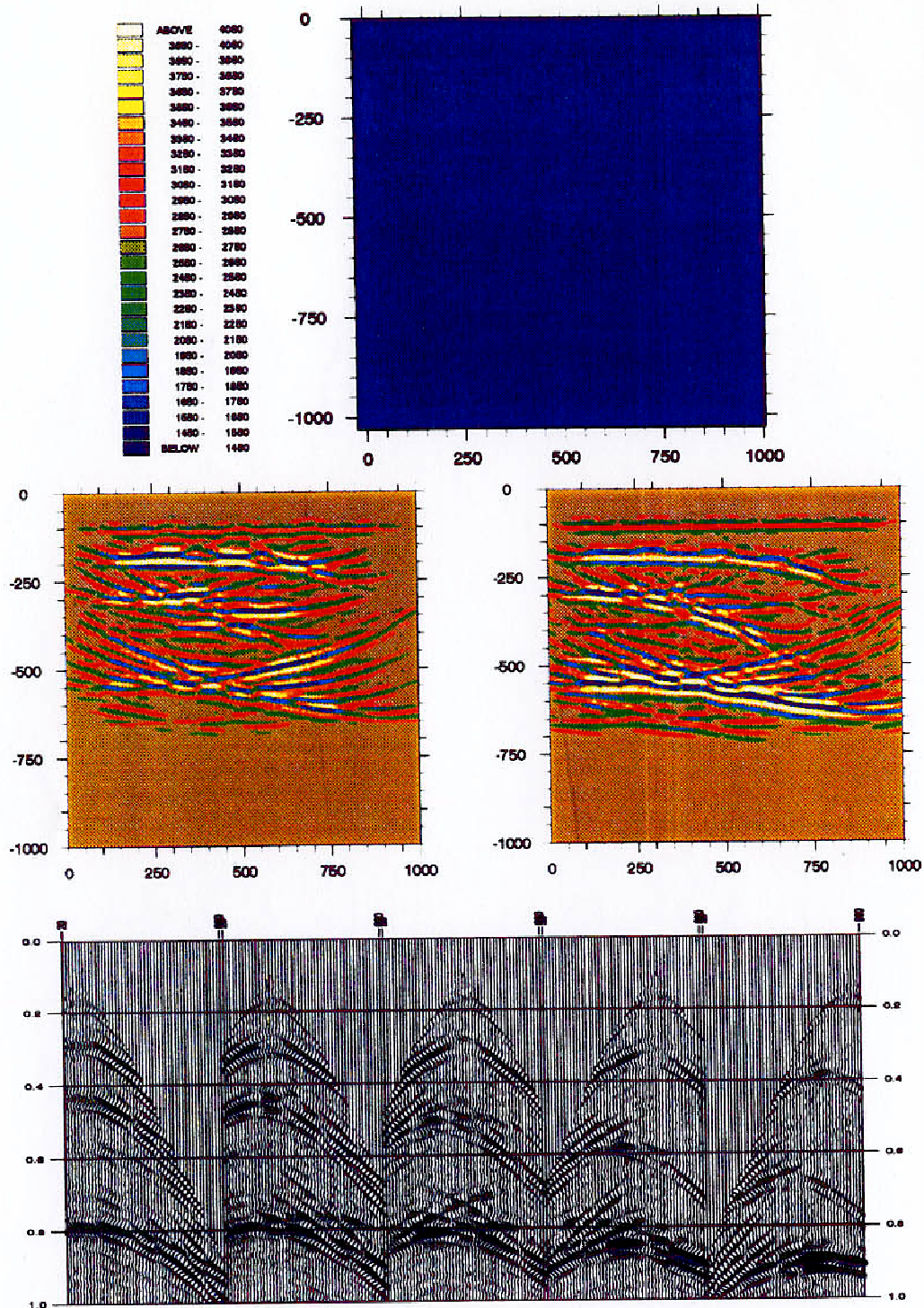
Fig. 5.3 Multishot resimulation with a uniform propagator of 1500 m/s. Top: uniform propagator 1500 m/s. Middle: intermediate stacked depth reflectivity with respect to \epsilon (left) and \sigma (right). Bottom: corresponding resimulation.
