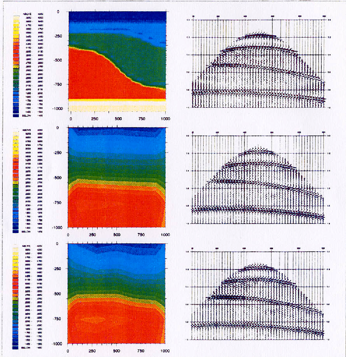
Fig. 4.2 Multiscale minimization with respect to \nu , with the true time reflectivity s(t) . Top: true velocity \nu_{\text{true}} , and data d = \varphi(\nu_{\text{true}}, \sigma) = \mathcal{M}\varphi(\nu_{\text{true}}, \bar{s}) . Then, left: velocities, and right: corresponding resimulations. Middle: after 3 hours of minimization on a Cray-2 on the 1st scale from the minimum on the 0th scale. Bottom: after 3 hours of minimization on a Cray-2 on the 2nd scale from the minimum on the 1st scale.
