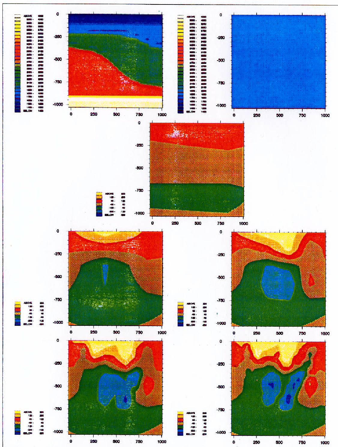
Fig. 5.5 Multishot: gradient with respect to the propagator. Top left: true propagator. Top right: uniform initial propagator 1800 m/s. Then, from left to right and from upper middle to bottom: gradient of the modified data misfit function \mathcal{M}\mathcal{J} with respect to the propagator successively projected on the 0th, 1st, 2nd, 3rd and 4th scale grids.
