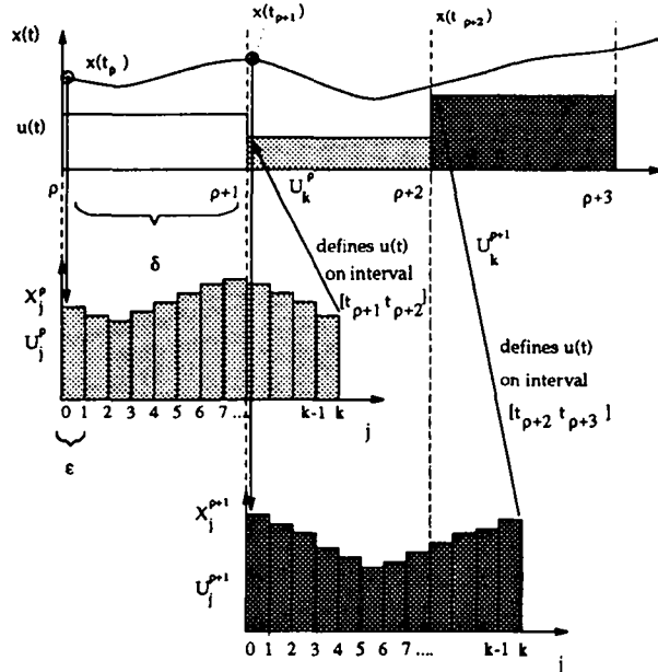
Figure 2.1 Representation of the HOC control strategy proposed in [1]. x(t) represents the state evolution of the controlled plant over time t . At each instant t_\rho , the plant is sampled and the vector x(t_\rho) is used as initial value X_0^\rho for system (2.14). The plot X_j^\rho, U_j^\rho represents the result of the numerical integration of system (2.14) for j = 0 to j = k . The control value of u over the interval t_{\rho+1} to t_{\rho+2} is chosen to be U_k^\rho . Clearly, to be implementable, the numerical integration of the DAE has to be faster than real-time.
