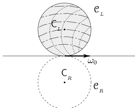
Figure 5 : Domain of type RL
