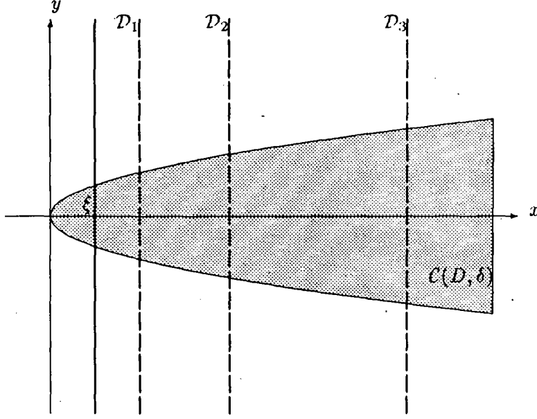
Figure 2: Illustration to the convex cone C(D, \delta) and the domains \mathcal{D}_m defined in Fact 4.
