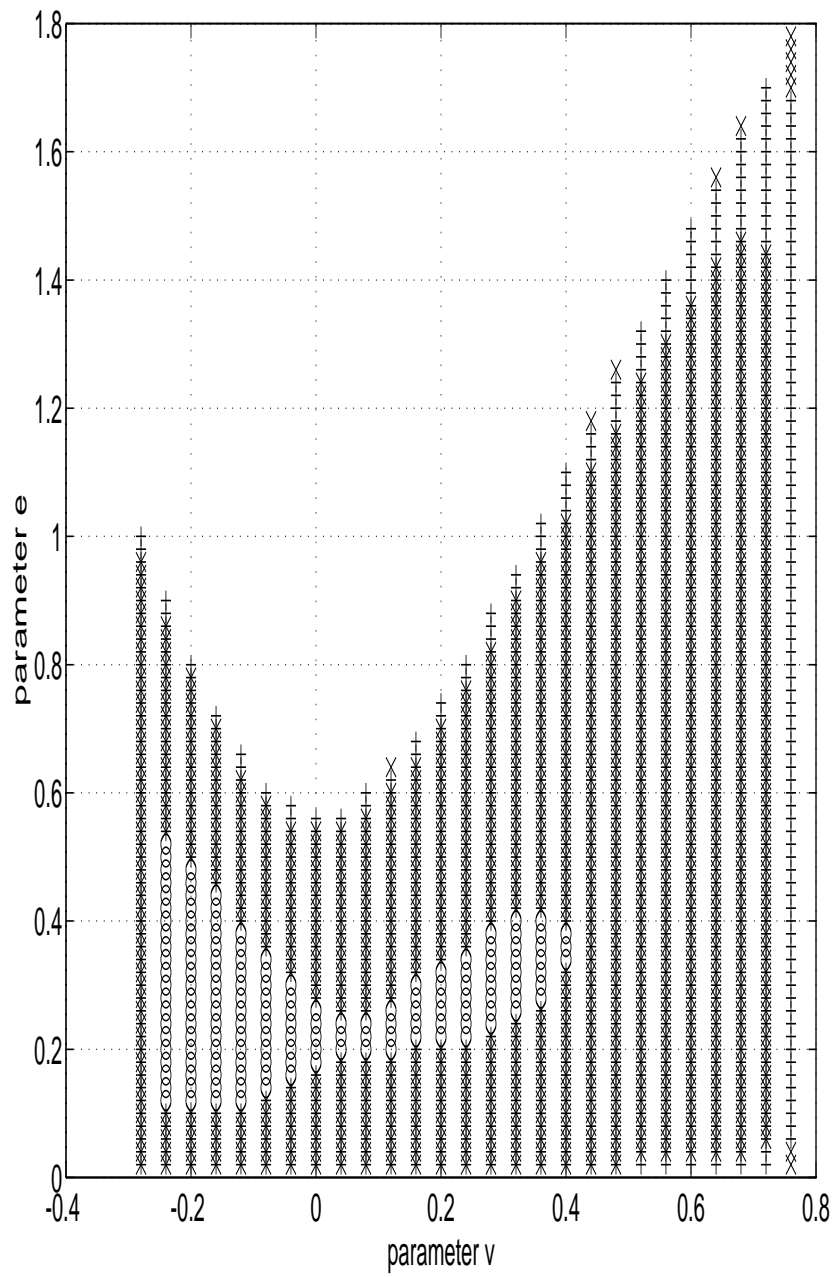
Figure 4: Asymptotic stability zone computed by using \alpha_0(A)
