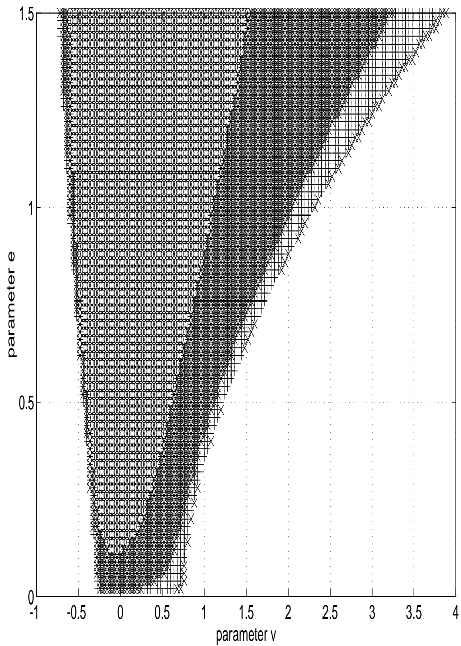
Figure 2: Asymptotic stability zone computed by using \alpha_0(A)
