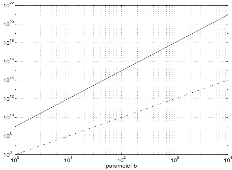
Figure 1: Graphs of the characteristics \alpha_0(A) and \alpha_{1/2}(A)
