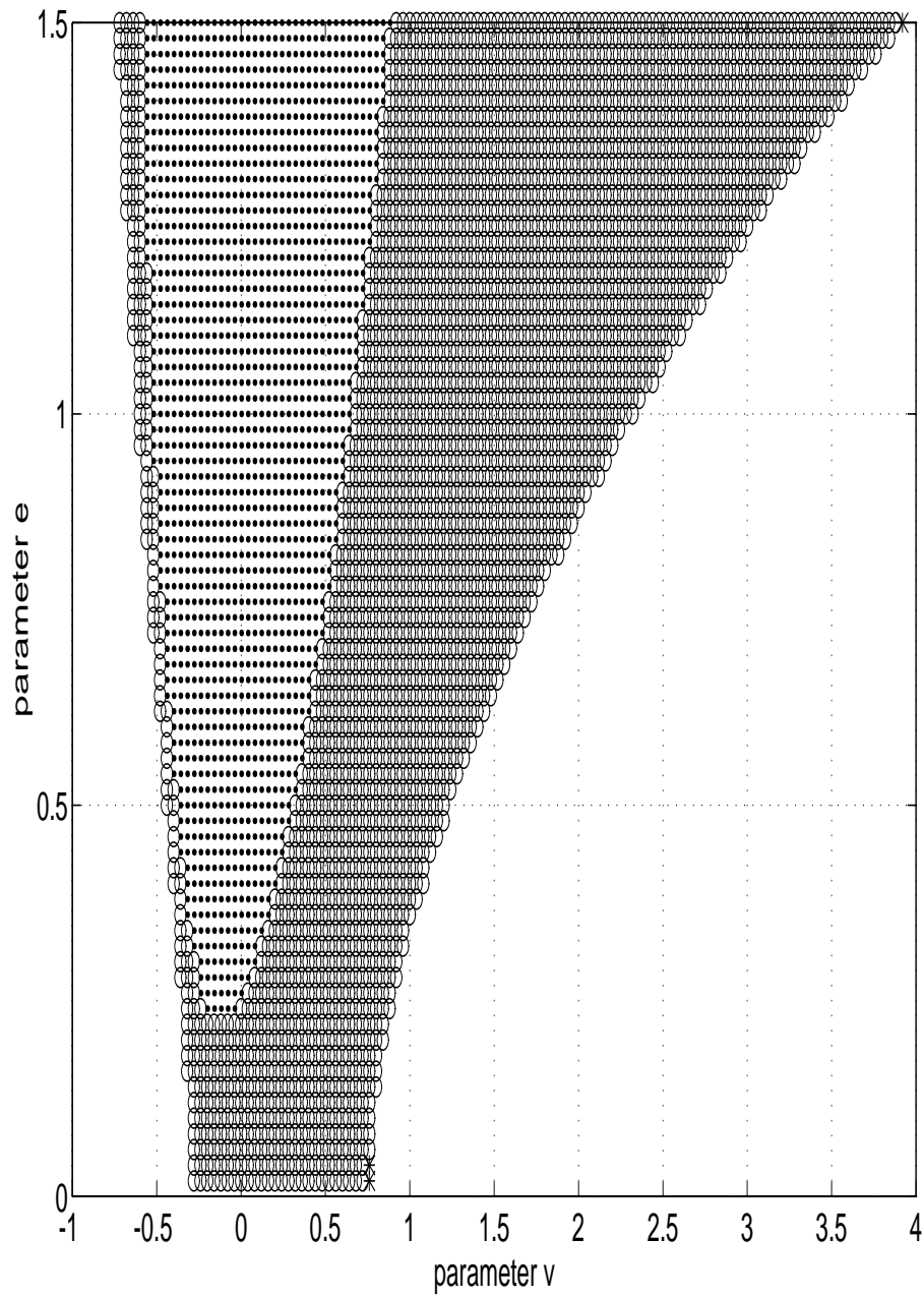
Figure 3: Asymptotic stability zone computed by using \alpha_{1/2}(A)
