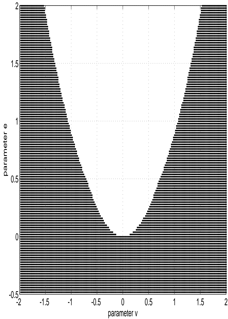
Figure 11: Asymptotic stability zone computed by using \alpha_{1/2}(A)
