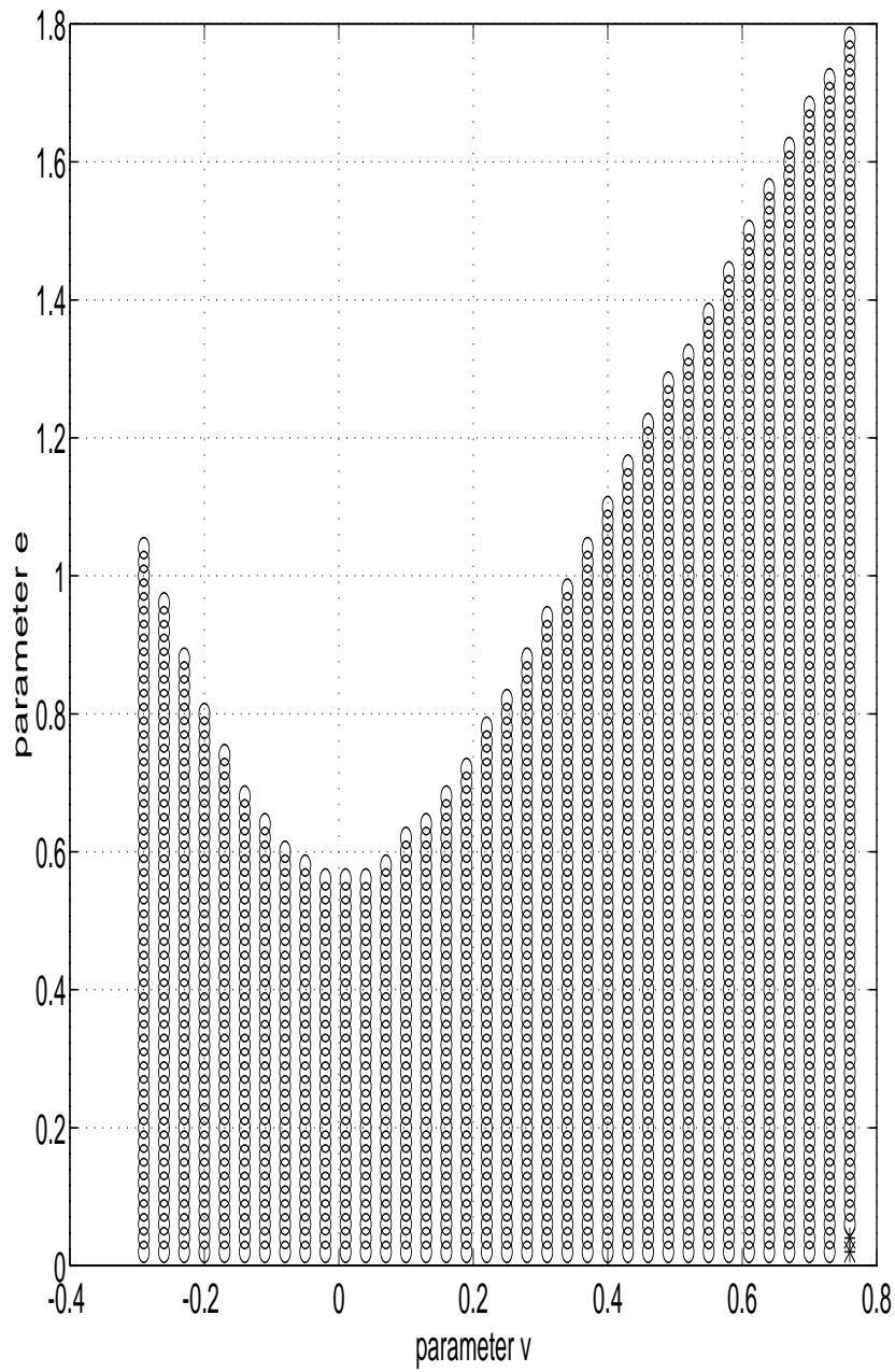
Figure 5: Asymptotic stability zone computed by using \alpha_{1/2}(A)
