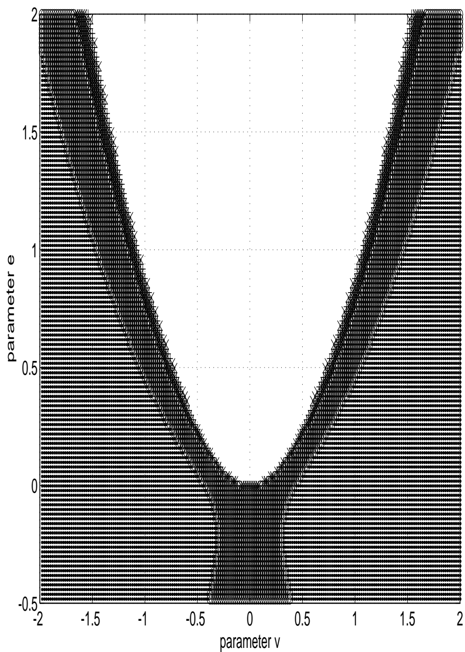
Figure 10: Asymptotic stability zone computed by using \alpha_0(A)
