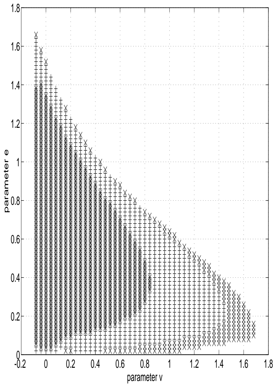
Figure 8: Asymptotic stability zone computed by using \alpha_0(A)
