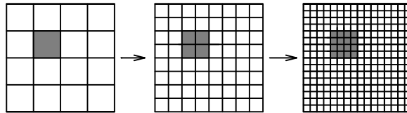
Figure 2: Multiresolution Scheme.
